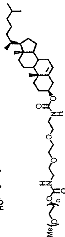
2KPEG-Chol (2%)
