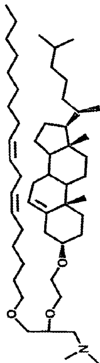
eCLinDMA (48%)
