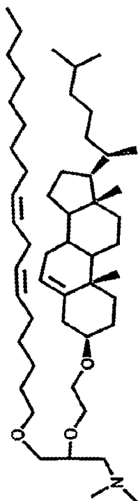
eCLinDMA (48%)
