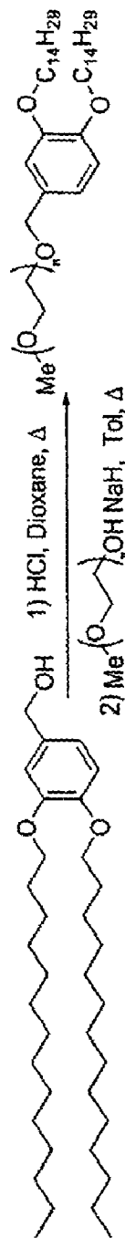
DMB-Peg
