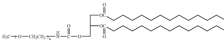
PEG-n-DMG structure
