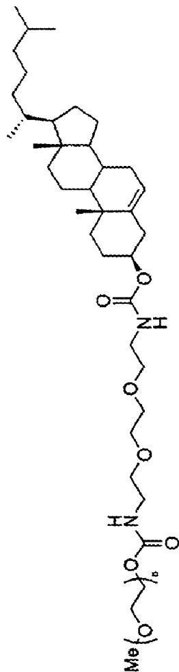
Cholesterol-PEG
