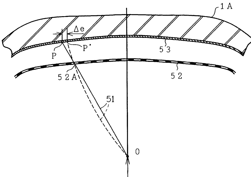
FIG. 5 (PRIOR ART)
