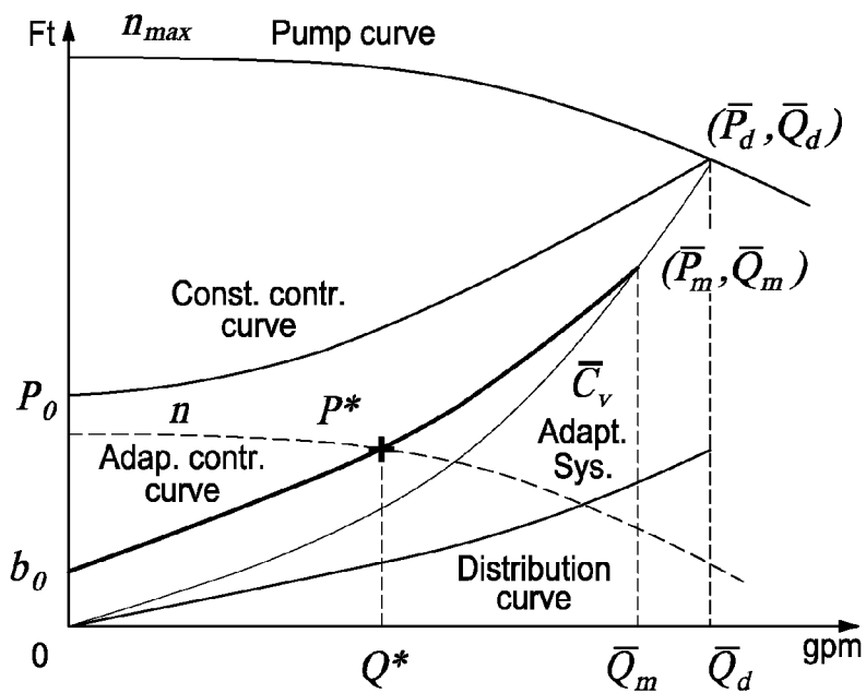
FIG. 2: A system and flow adaptive pumping control scheme for a hydronic pumping system.
