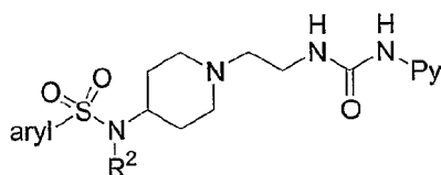
General formula 6
