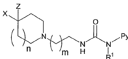
General Formula 2
