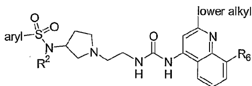
General formula 19
