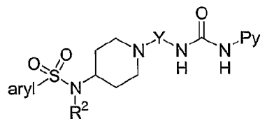
General formula 5
