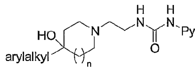
General formula 4
