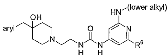
General formula 16
