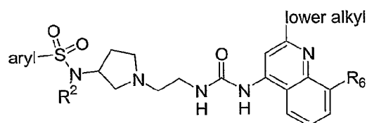
General formula 19
