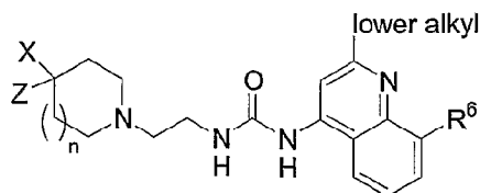
General formula 12
