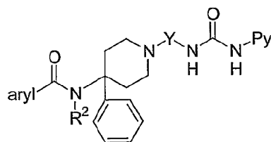
General formula 7
