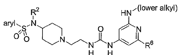
General formula 18
