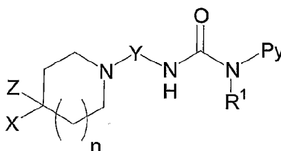
General Formula 1
