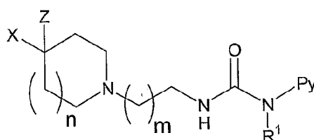
General Formula 2
