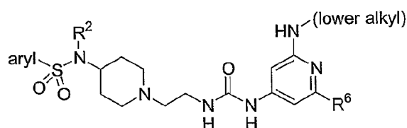
General formula 18
