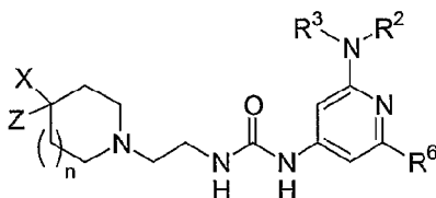
General formula 14
