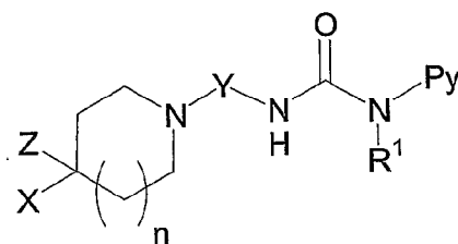
General Formula 1
