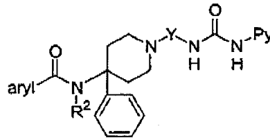
General formula 7
