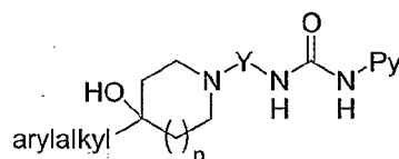
General formula 3
