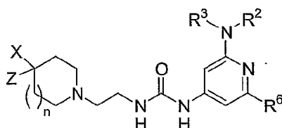
General formula 14
