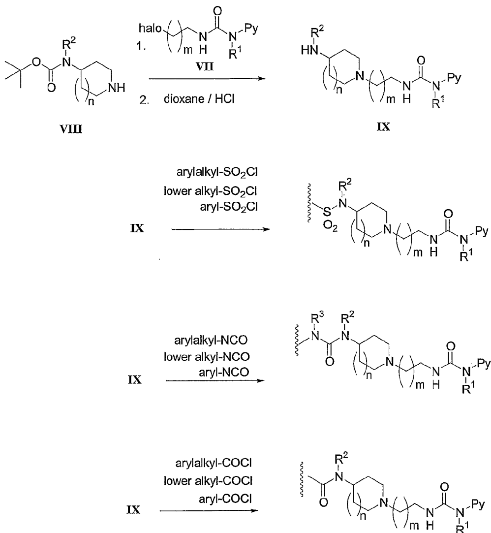
Scheme D
