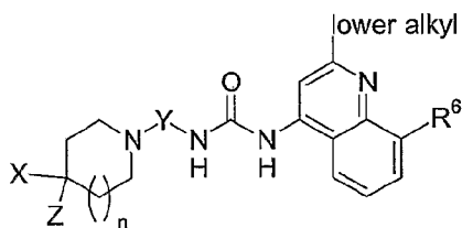
General formula 11
