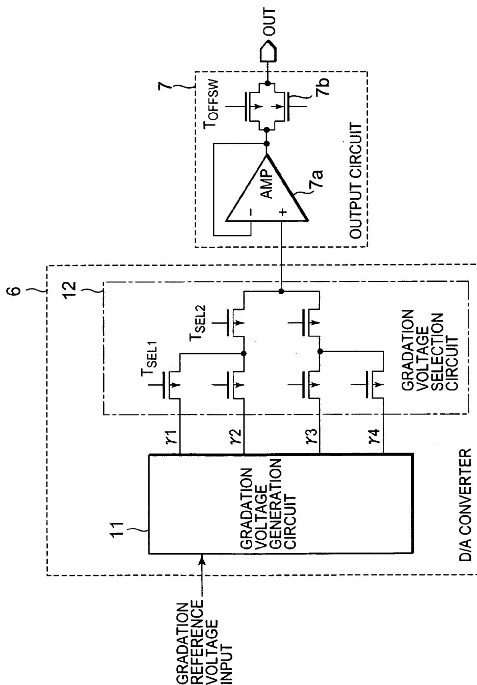
Fig. 7 PRIOR ART
