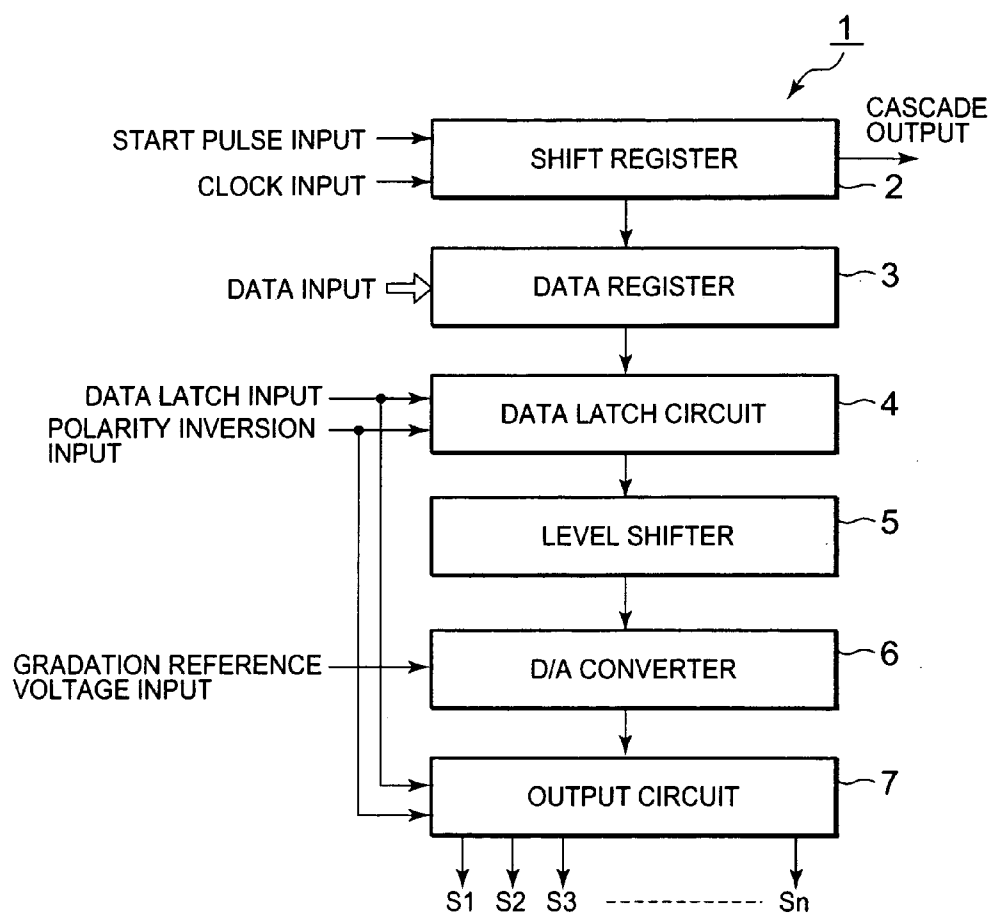
Fig. 5 PRIOR ART
