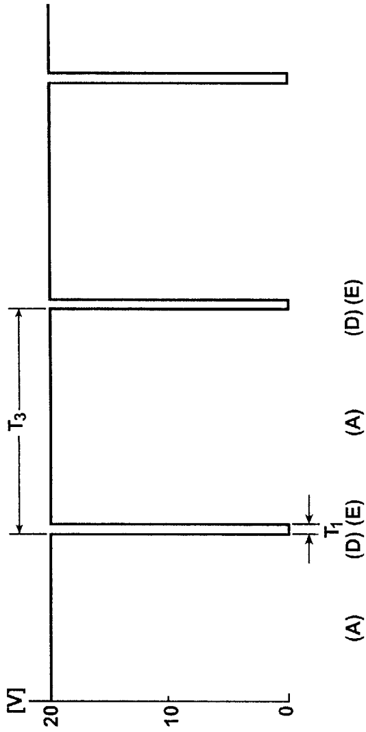
First Laminated Piezoelectric Element 45 (Discharging Side)
