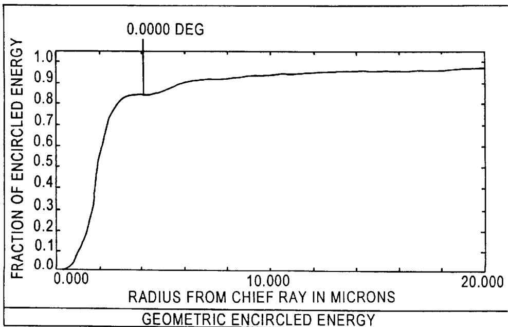
Defocus 0 \mu\text{m}
