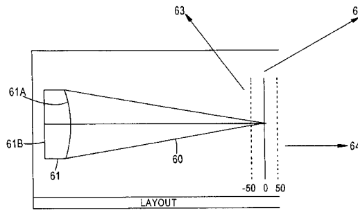
Optical Layout
