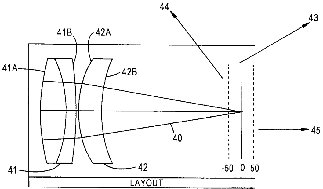
Optical Layout
