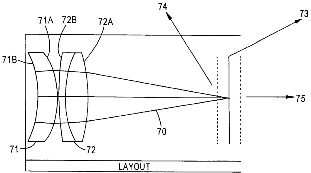
Optical Layout
