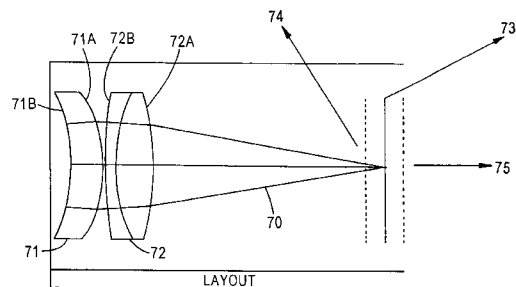
Optical Layout
