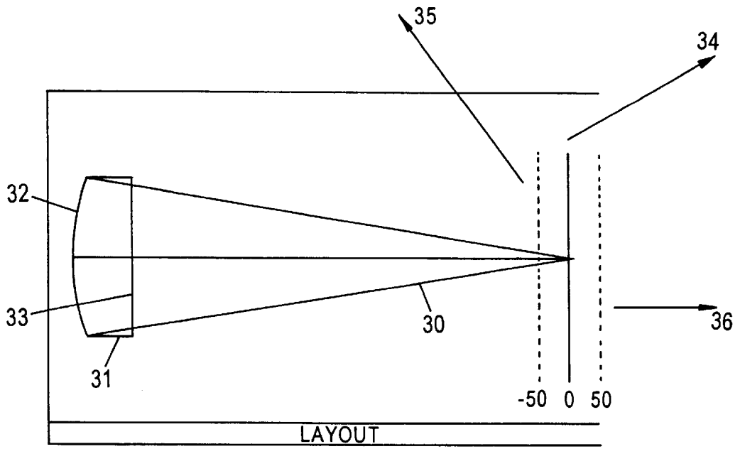
Optical Layout
