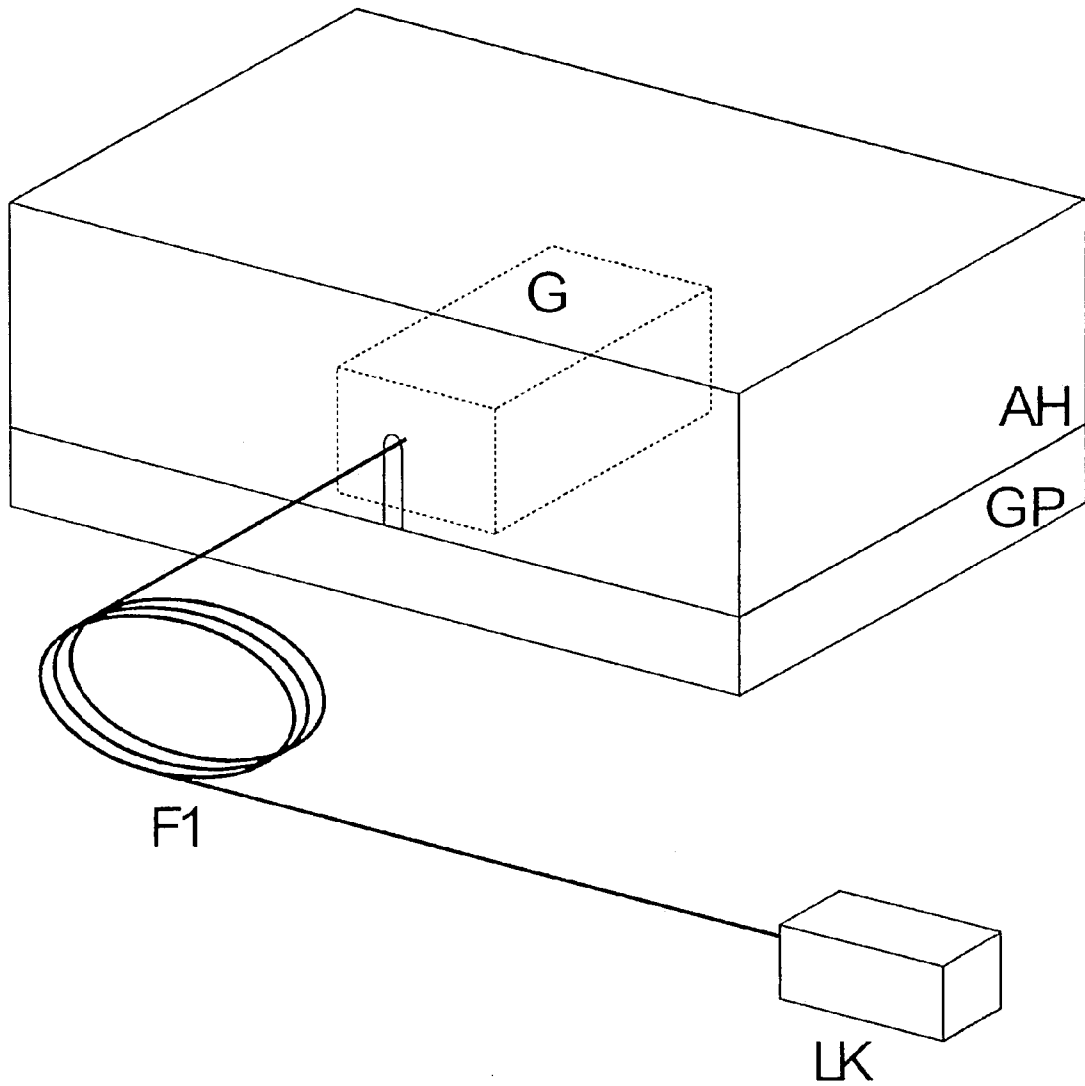
Figure 5: User port installed in the laser module
