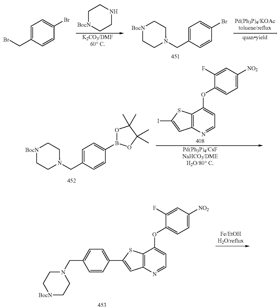
Scheme 89
