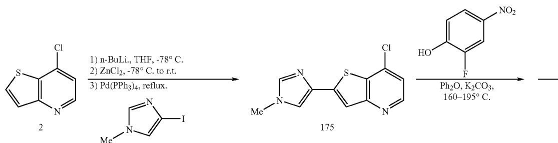
Scheme 35
