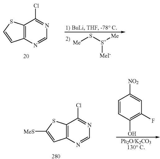
Scheme 64
