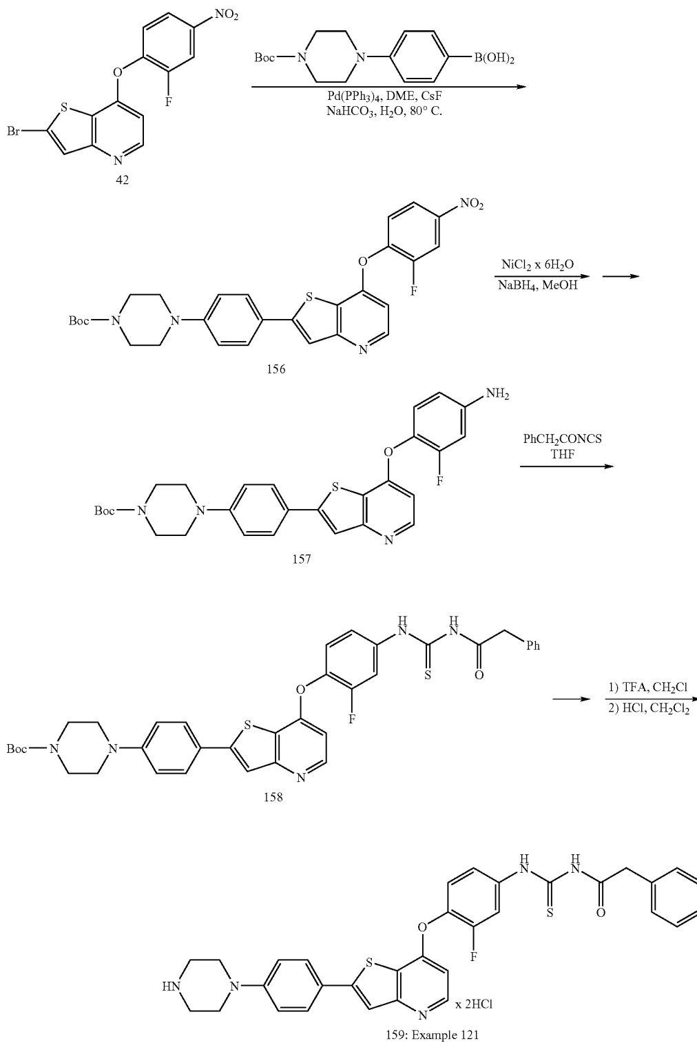
Scheme 30
