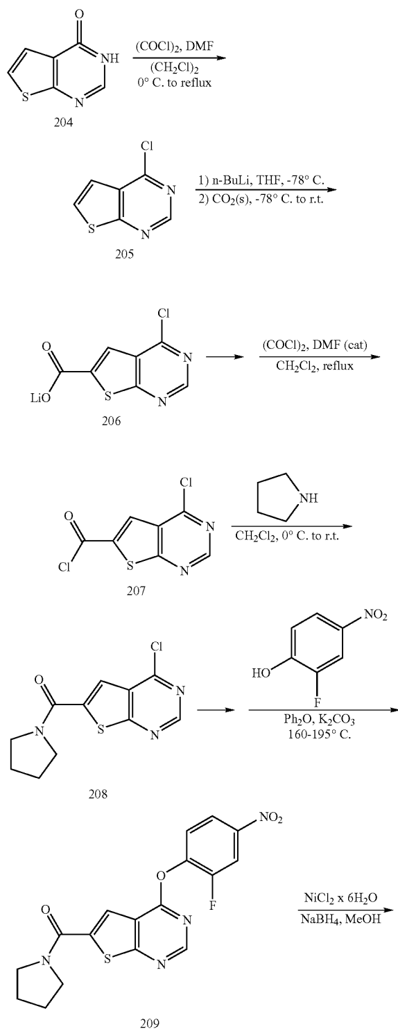
Scheme 44
