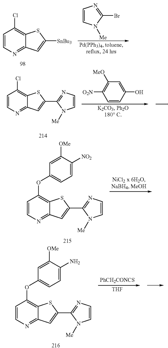
Scheme 46
