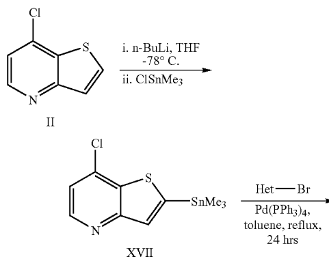
Scheme C
