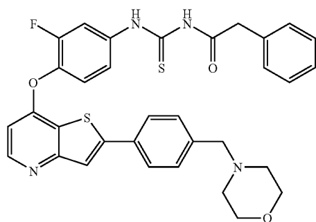
55: Example 56
