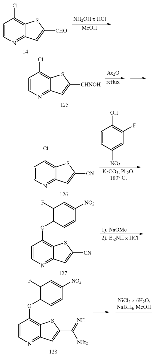
Scheme 23
