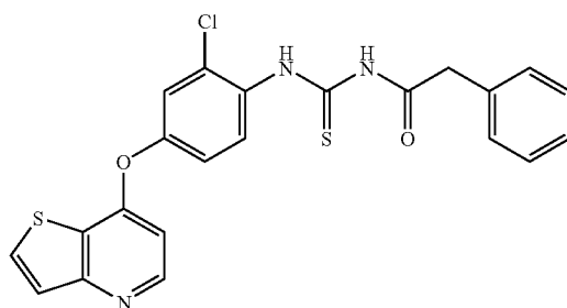
170b: Example 134
