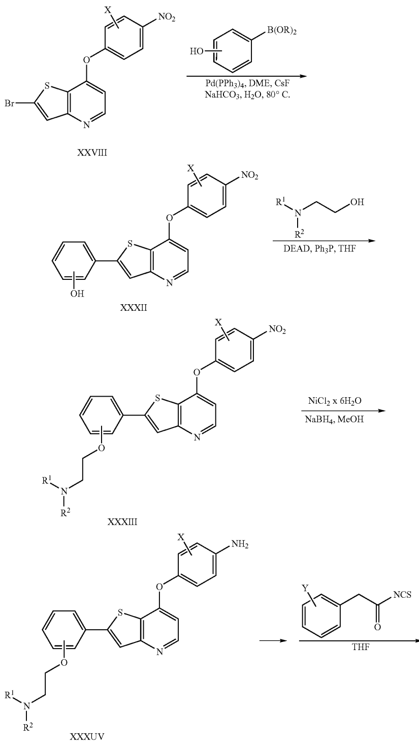
Scheme F
