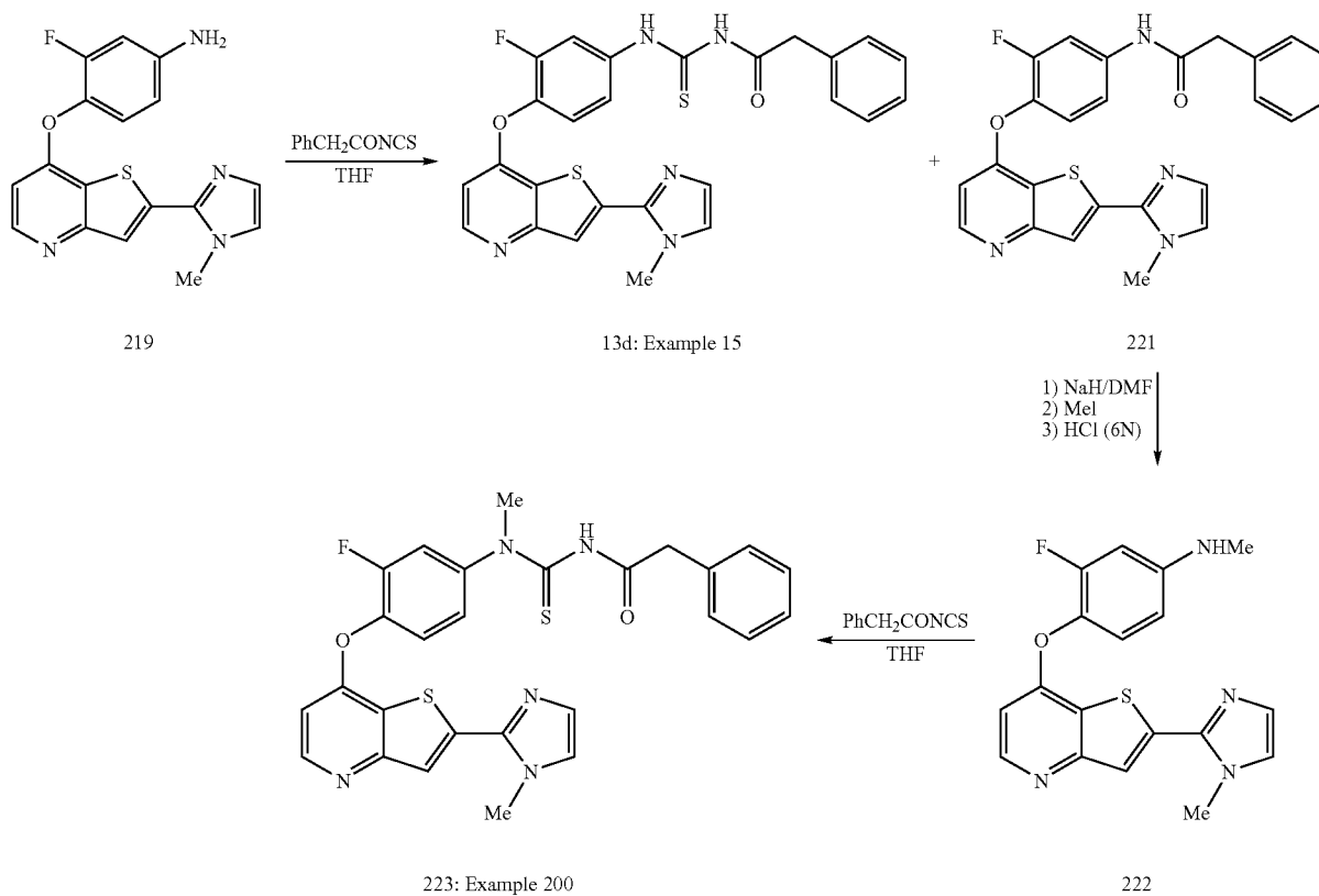
Scheme 48
