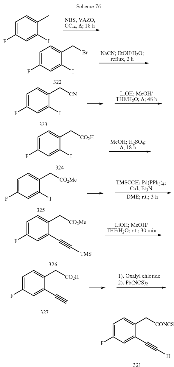
2-(2-Ethynyl-4-fluorophenyl)acetyl isothiocyanate (321)
