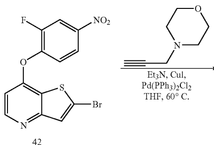
Scheme 12
