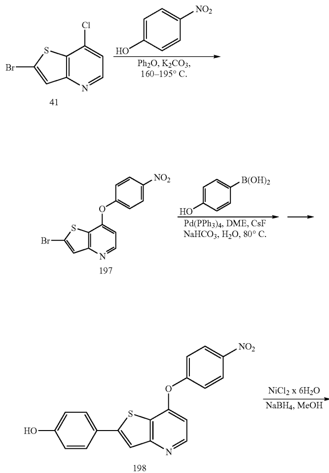
Scheme 42
