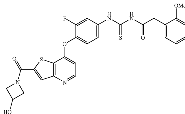
300: Example 230
