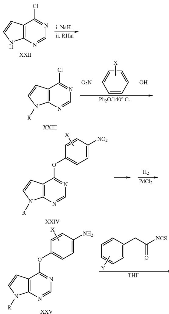
Scheme D
