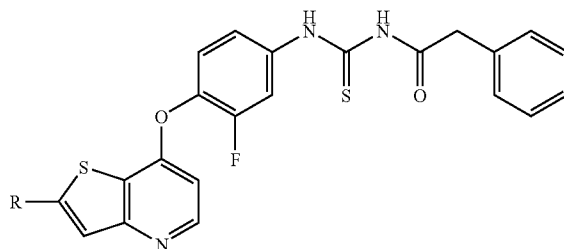
163a-h: Example 122-128
