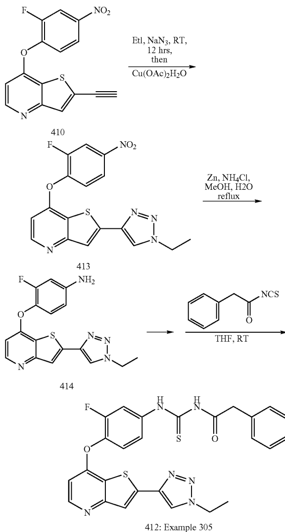
Scheme 83
