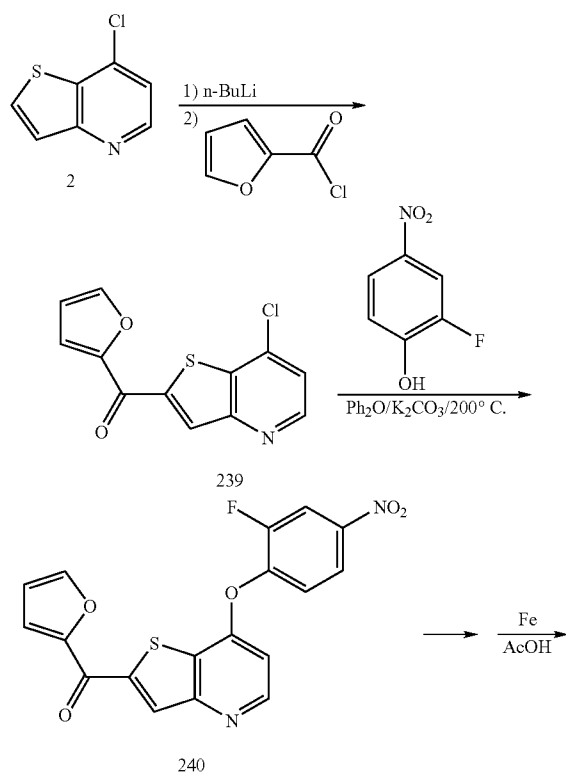
Scheme 53
