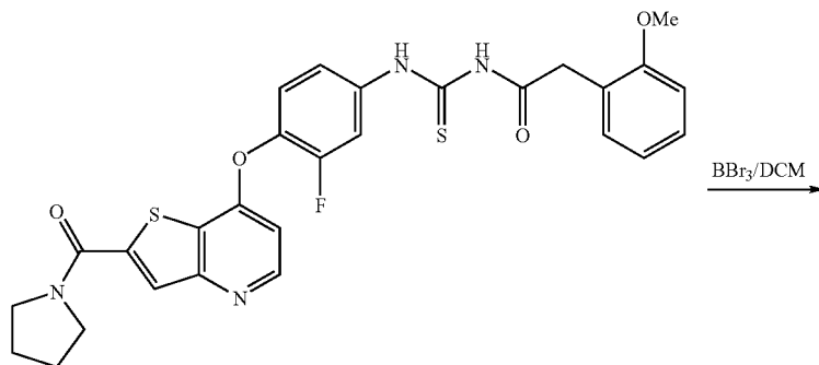
Scheme 41
