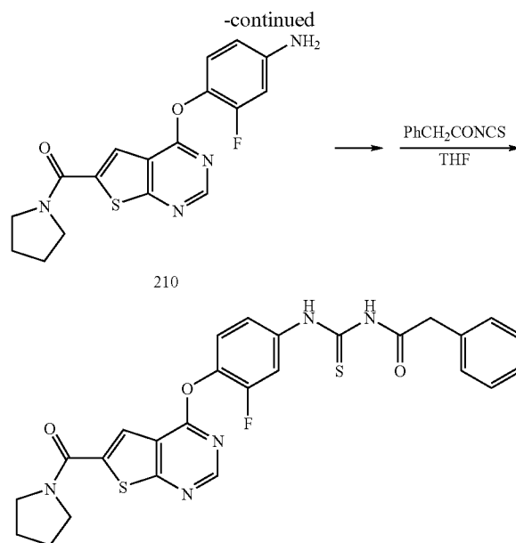
211: Example 187
