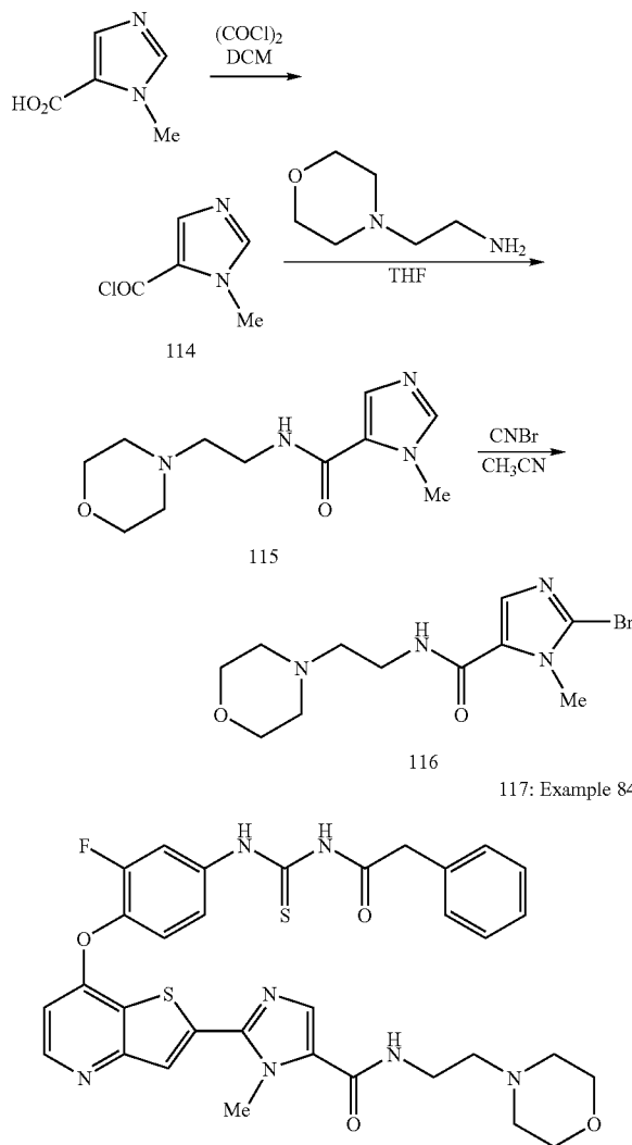
Scheme 21
