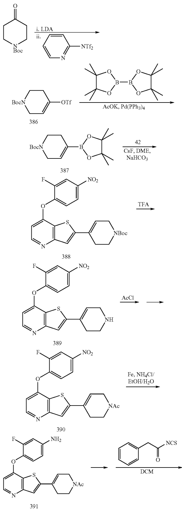
Scheme 81
