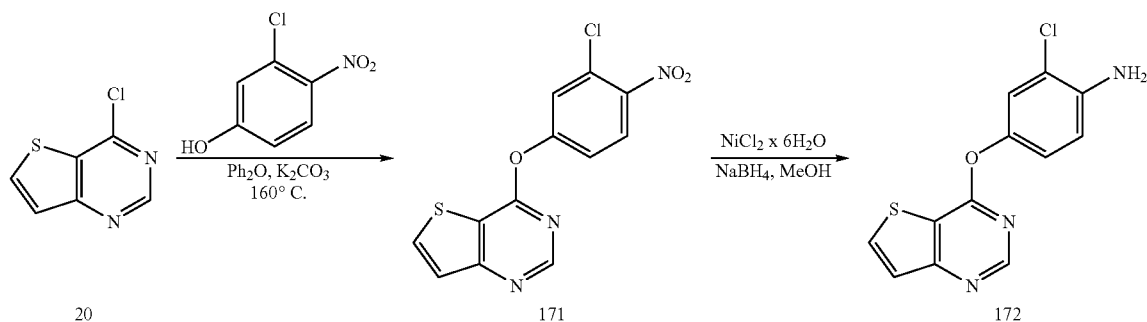
Scheme 34
