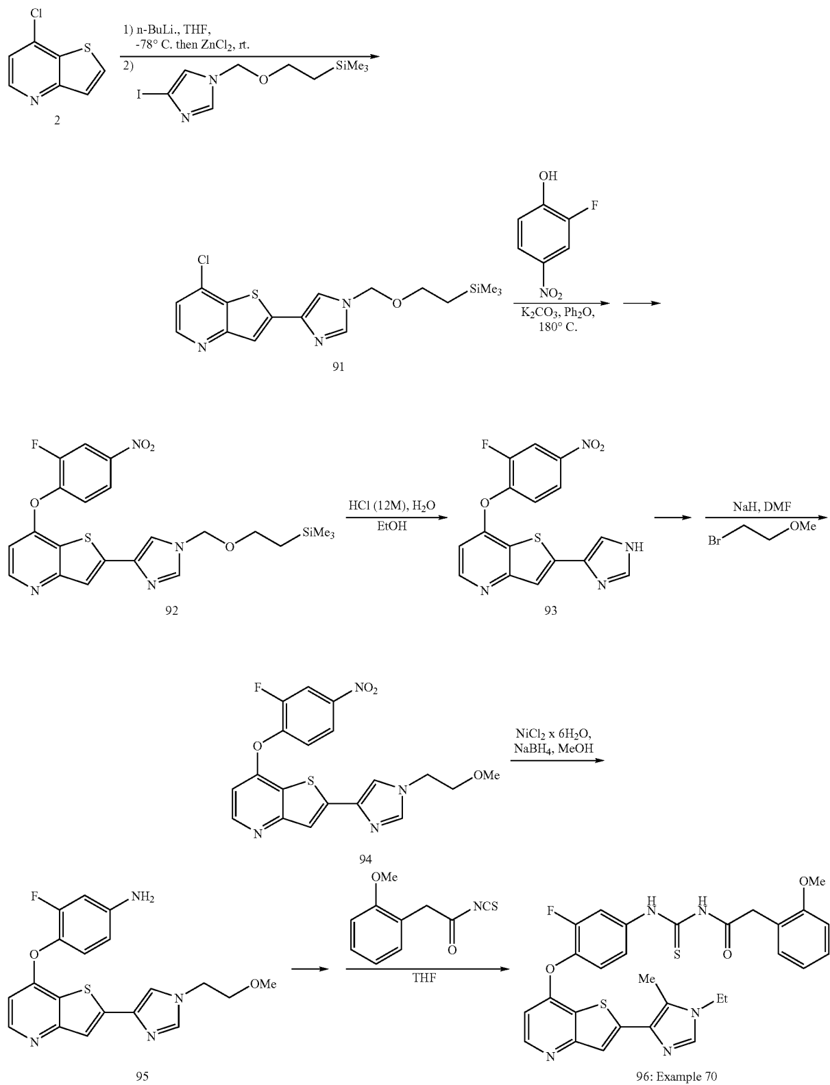
Scheme 18
