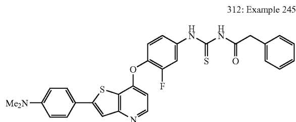
N-(4-(2-(4-(Dimethylamino)phenyl)thieno[3,2-b]pyridin-7-yloxy)-3-fluorophenyl)carbamothioyl)-2-phenylacetamide (312)
