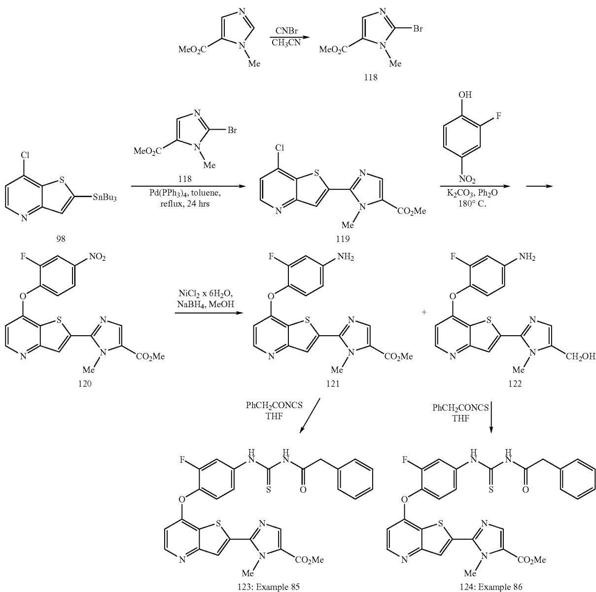
Scheme 22
