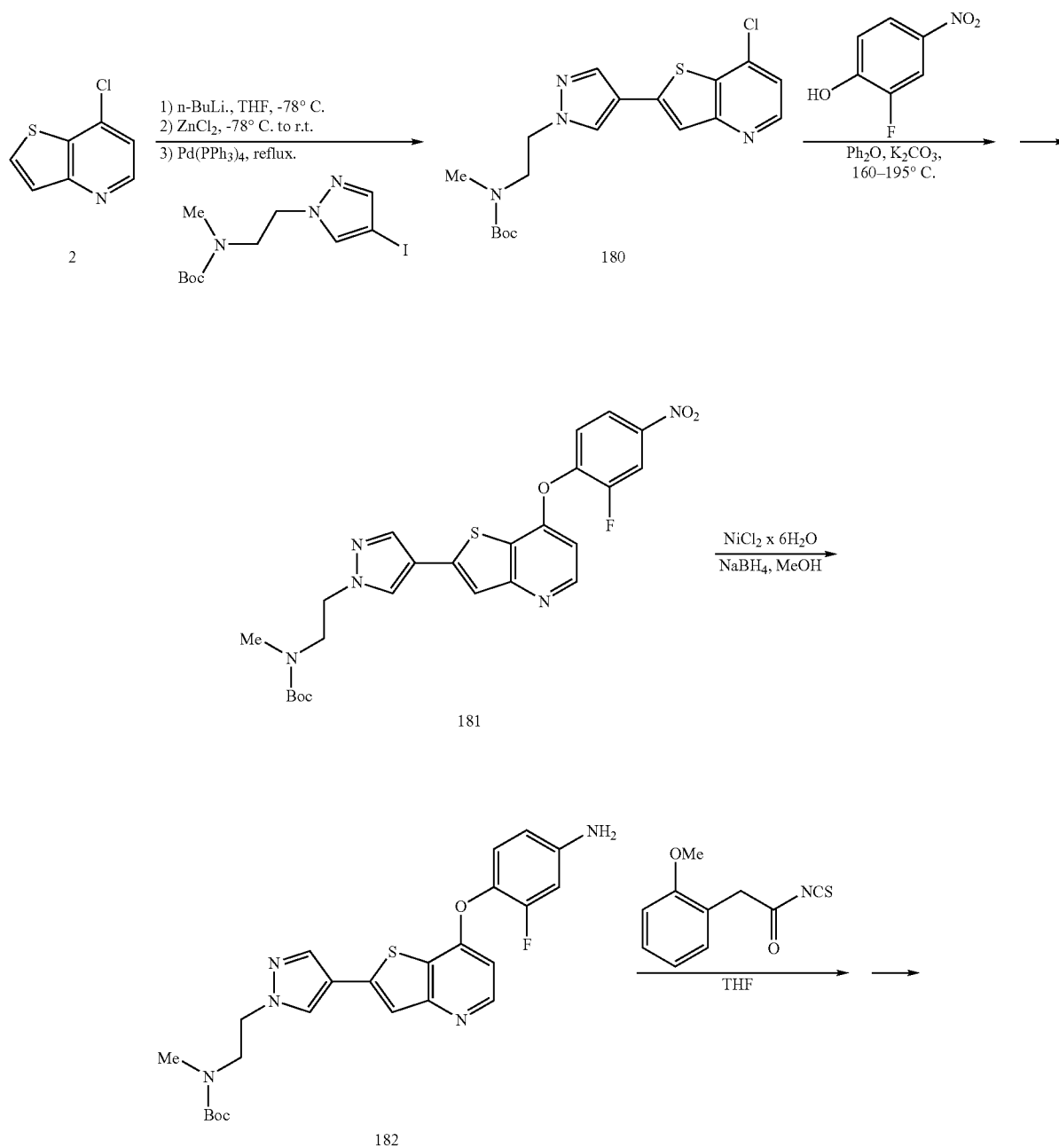
Scheme 26
