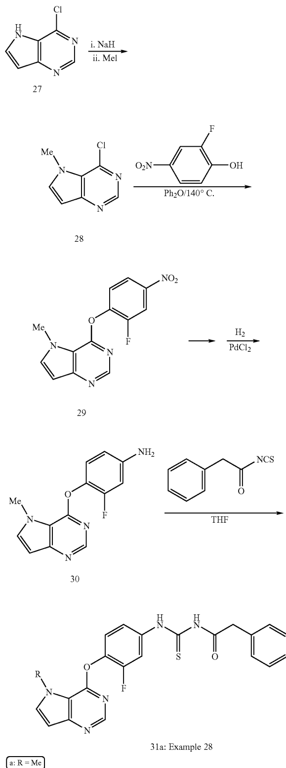
Scheme 5
