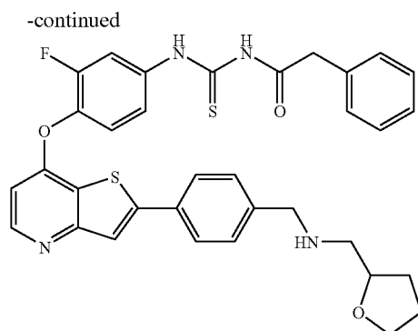
81: Example 66
