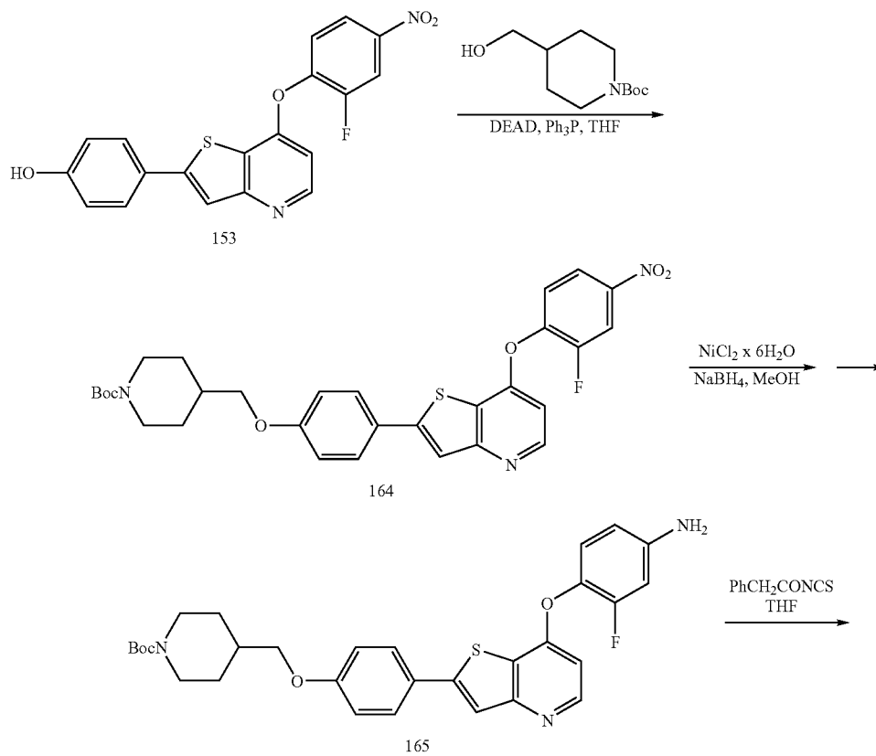
Scheme 32
