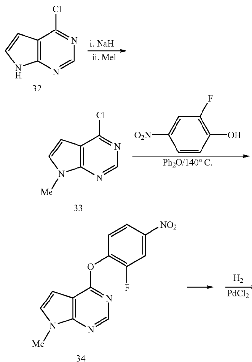
Scheme 6
