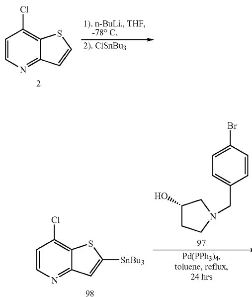
Scheme 19
