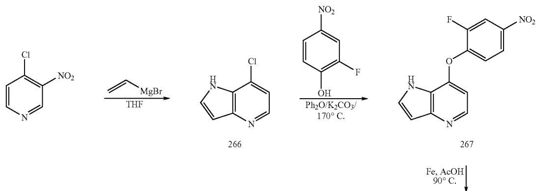
Scheme 61
