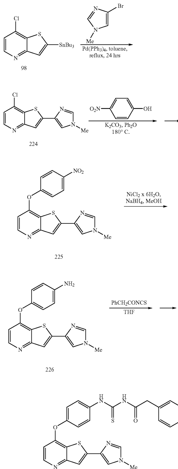
Scheme 49
