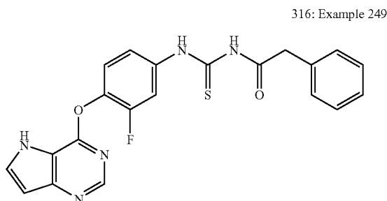
N-(4-(5H-Pyrrolo [3,2-d]pyrimidin-4-yloxy)-3-fluorophenylcarbamothioyl)-2-phenylacetamide (316)
