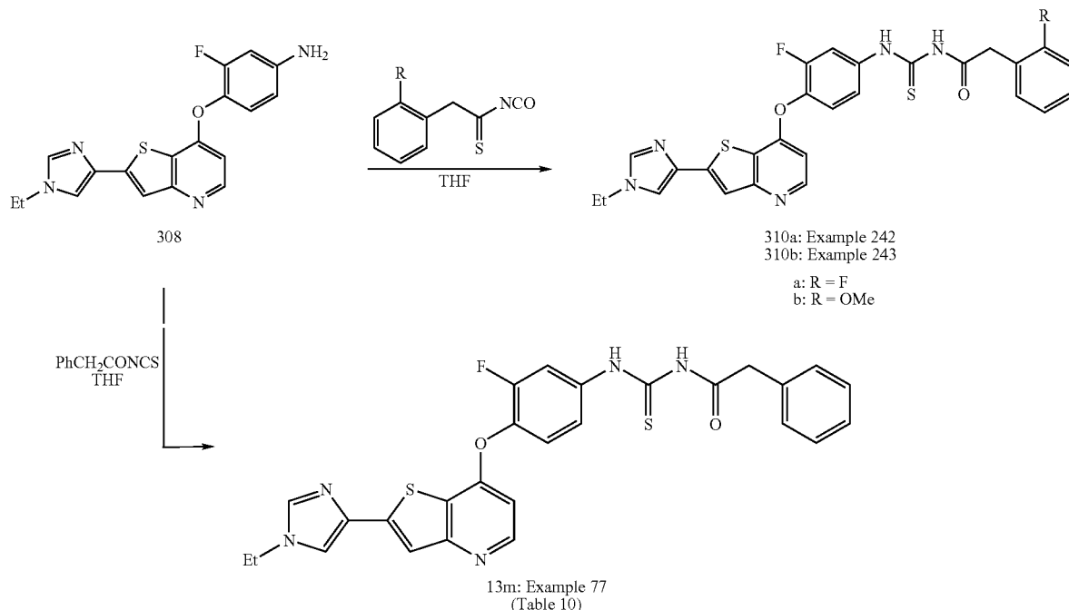
Scheme 74
