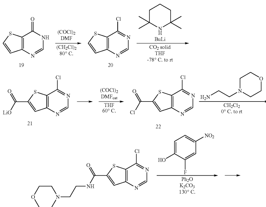
Scheme 4
