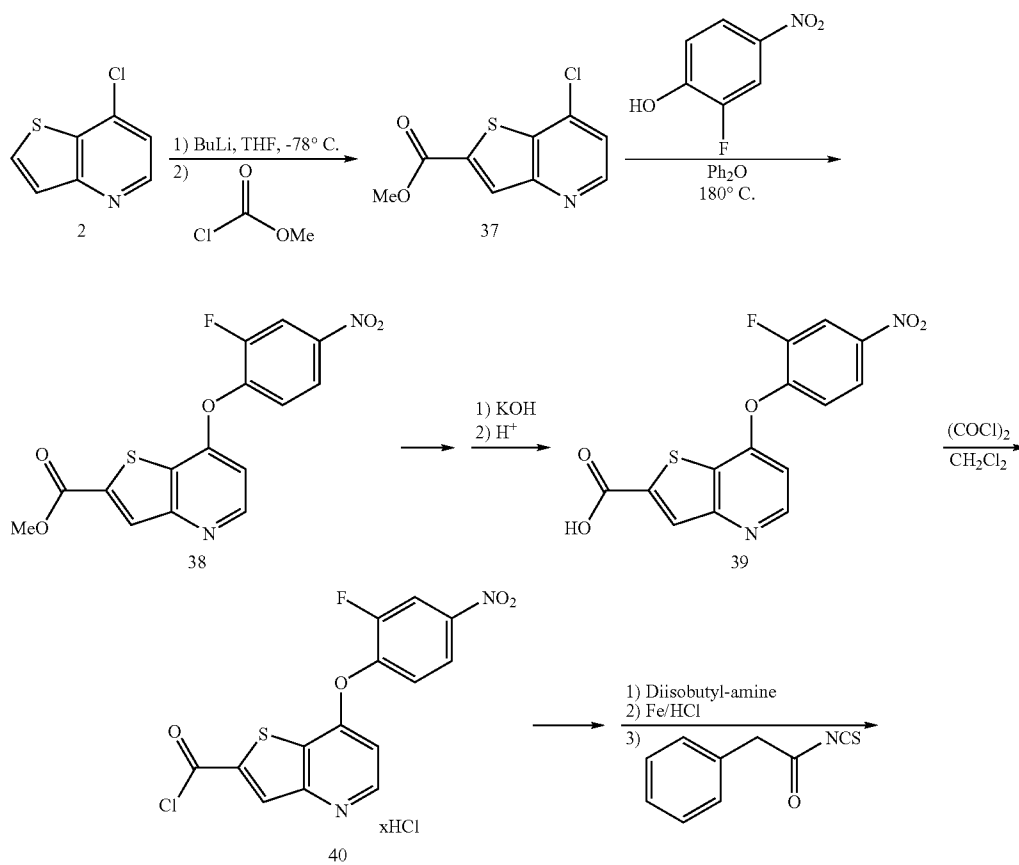
Scheme 7
