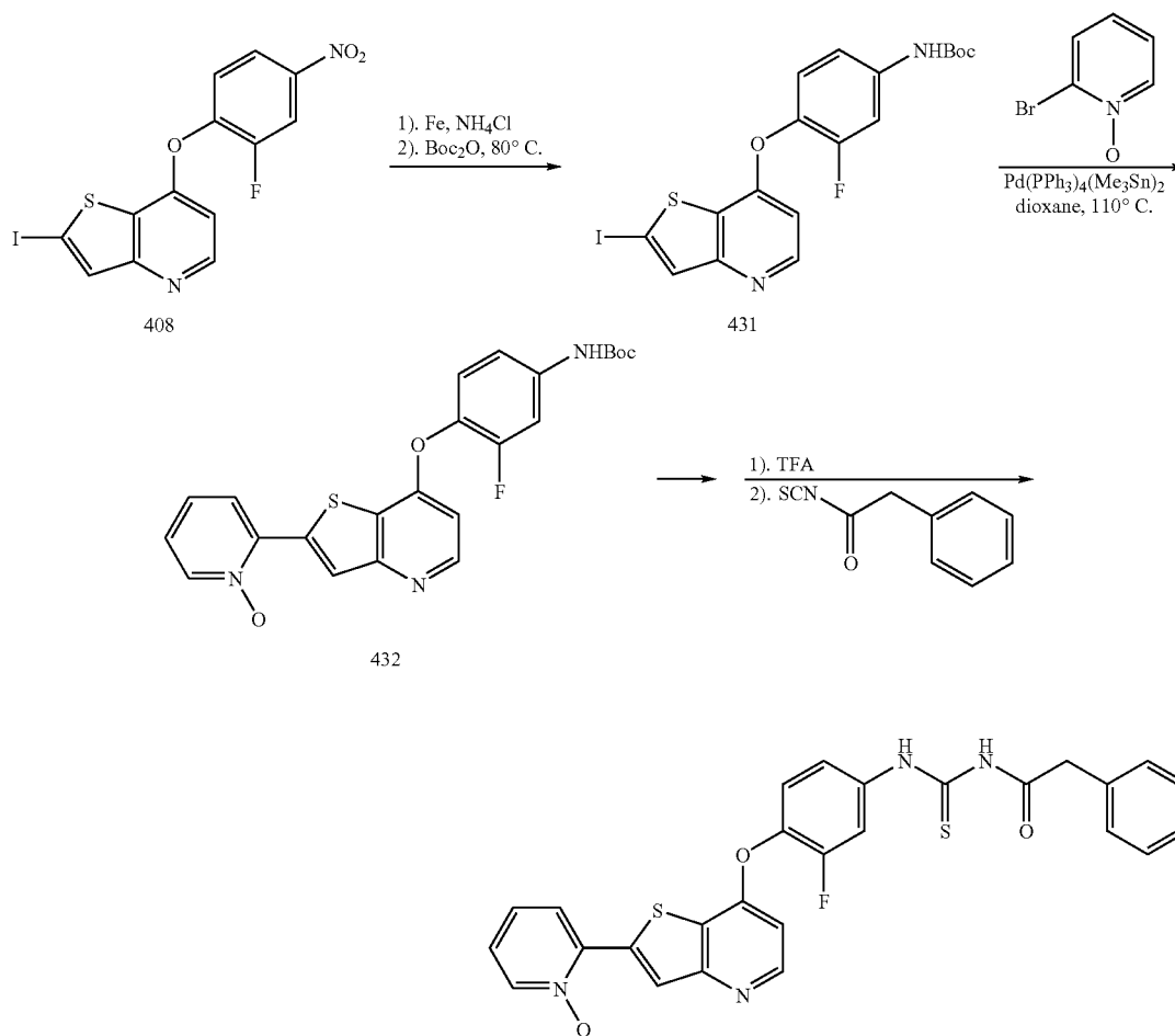
Scheme 86
