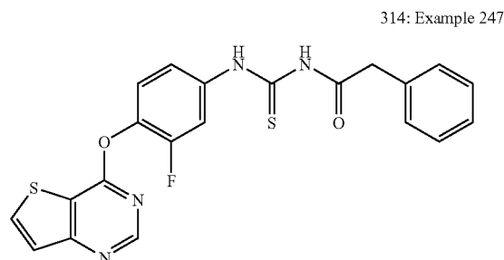
N-(3-Fluoro-4-(thieno[3,2-d]pyrimidin-4-yloxy)phenyl)carbamothioyl)-2-phenylacetamide (314)
