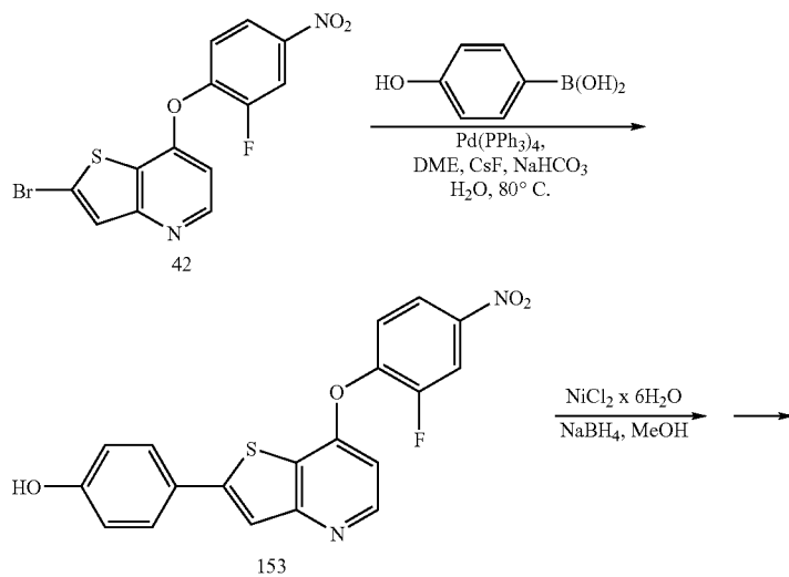
Scheme 28
