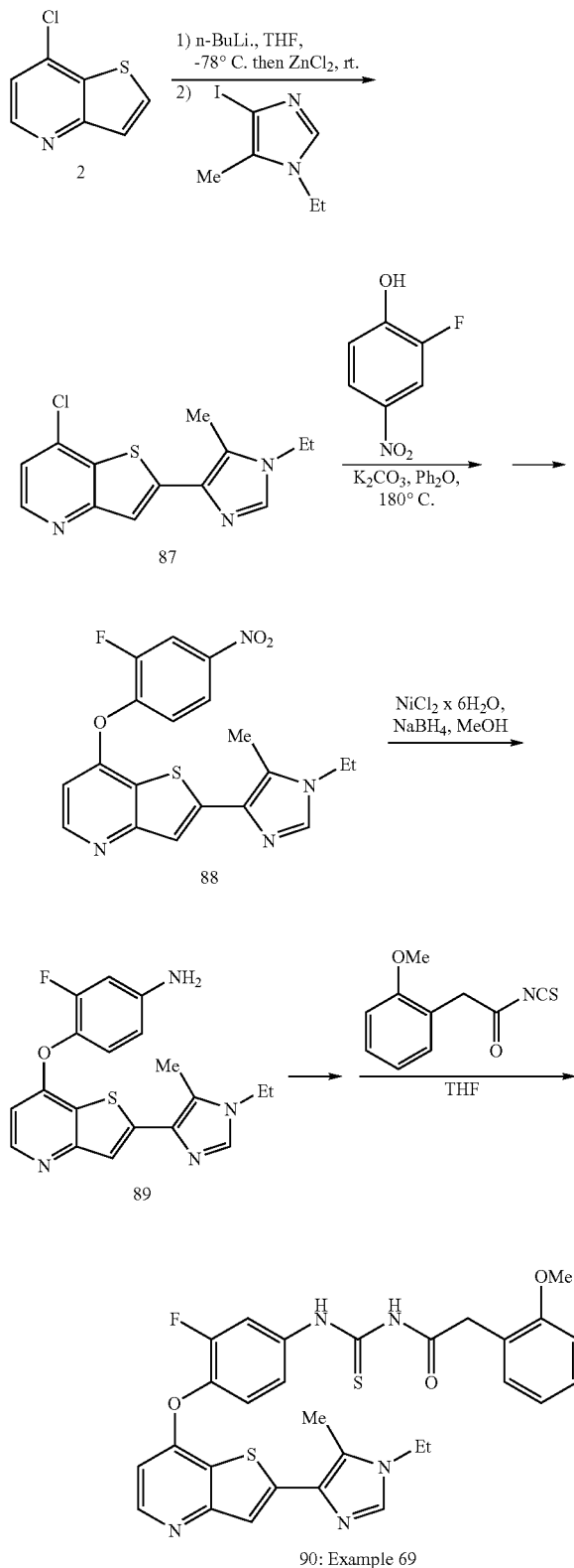
Scheme 17
