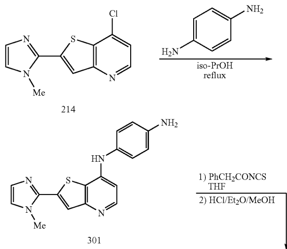
Scheme 69
