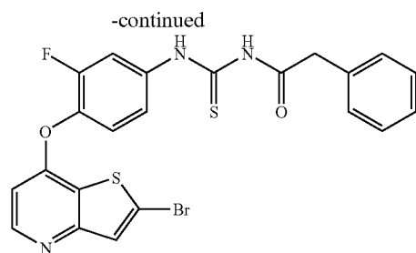
44: Example 48
