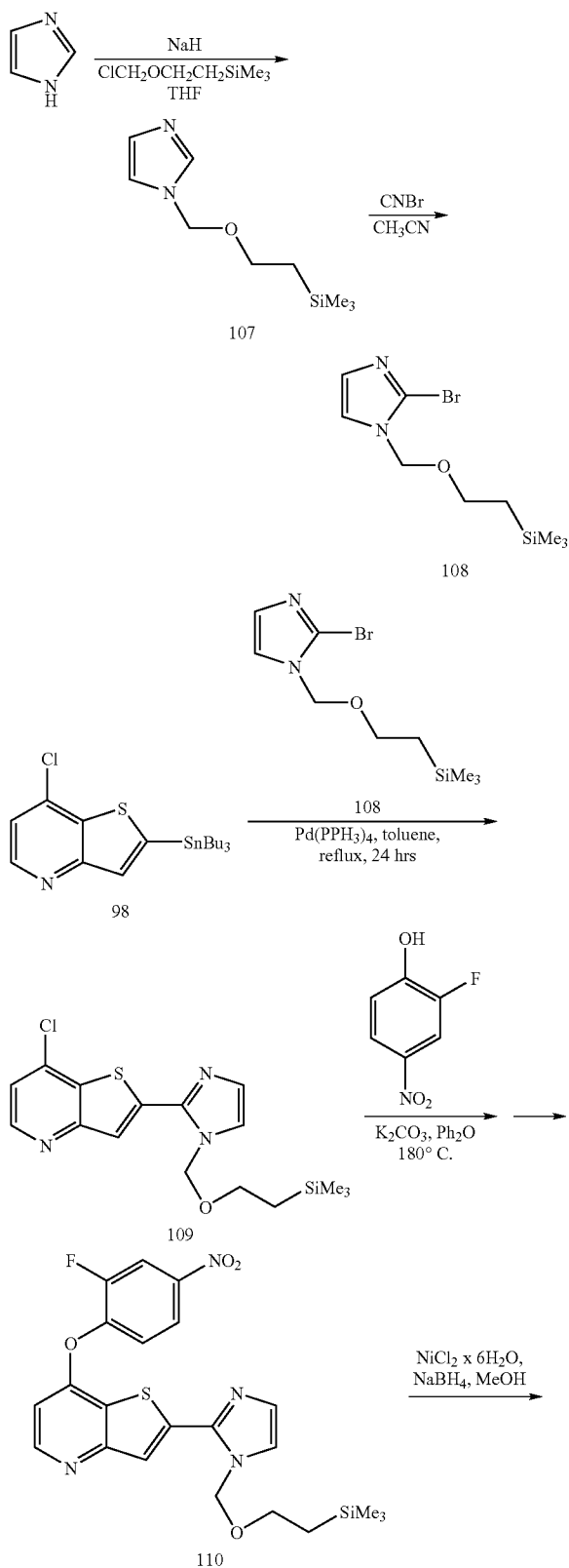
Scheme 20
