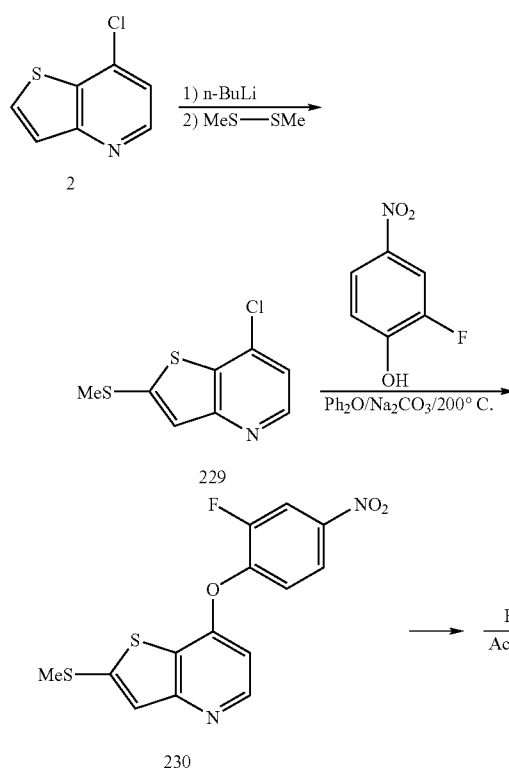
Scheme 50
