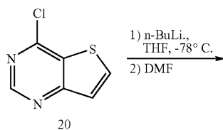
Scheme 37
