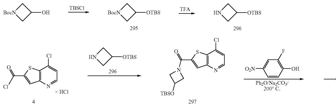
Scheme 68
