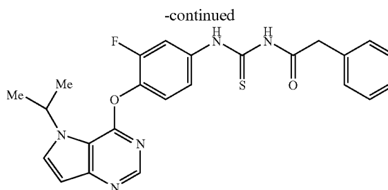
249: Example 211
