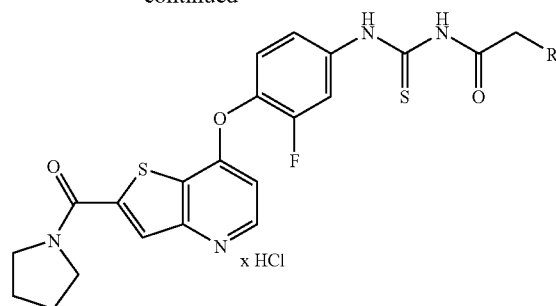
196a: Example 182
