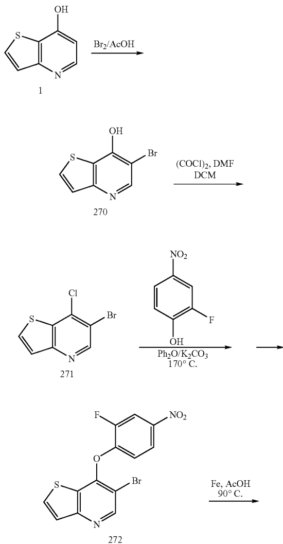
Scheme 62
