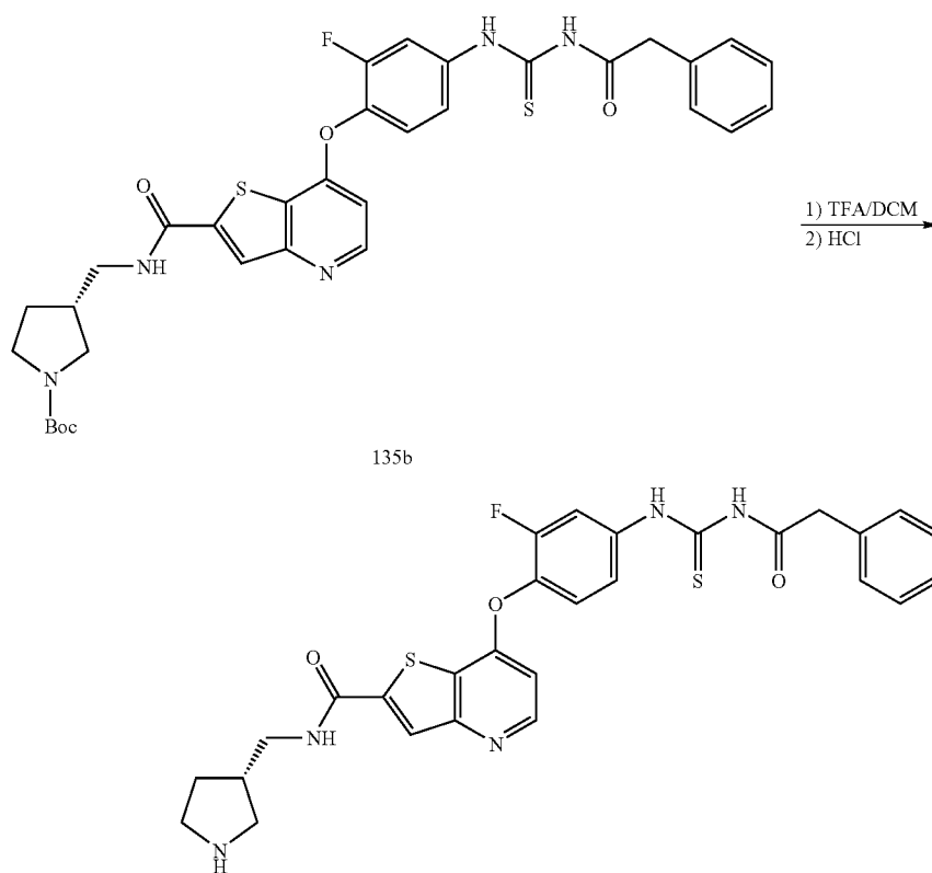
Scheme 25
