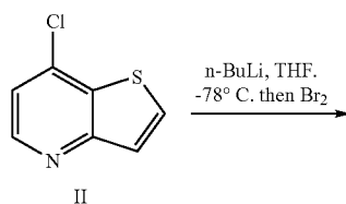
Scheme E
