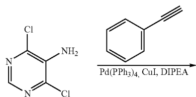
Scheme 57
