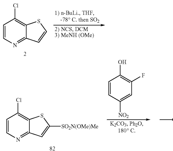
Scheme 16a
