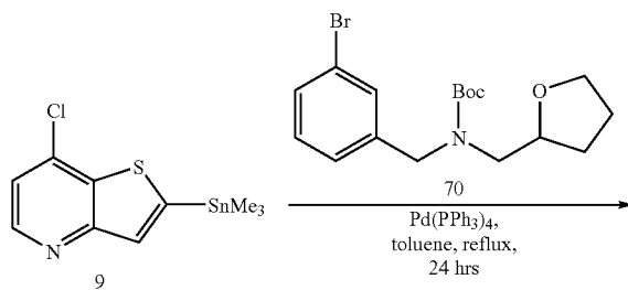
Scheme 16
