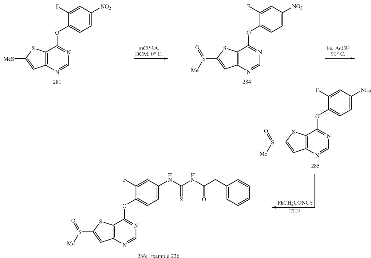
Scheme 65
