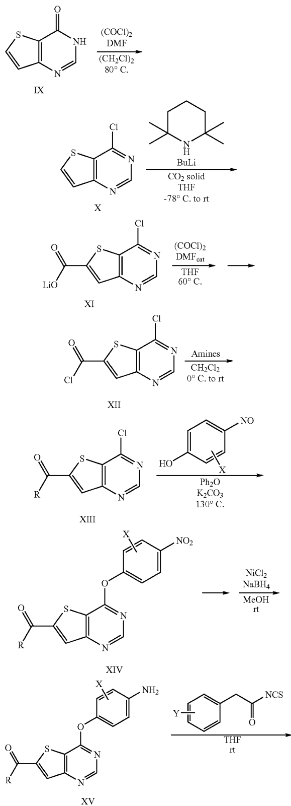
Scheme B
