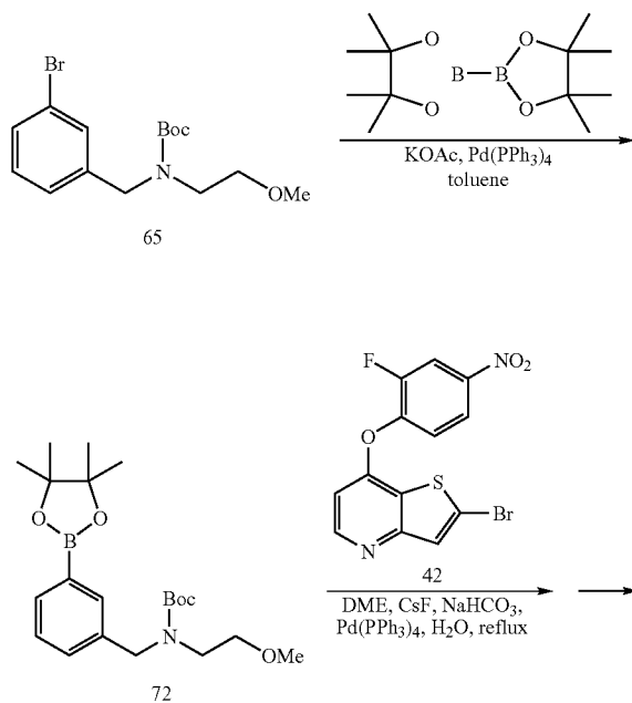
Scheme 15
