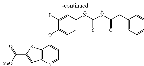
288: Example 227
