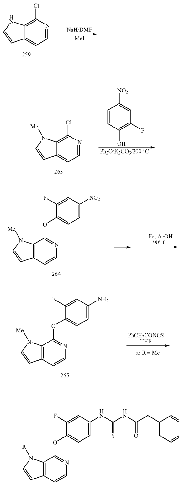
Scheme 60
