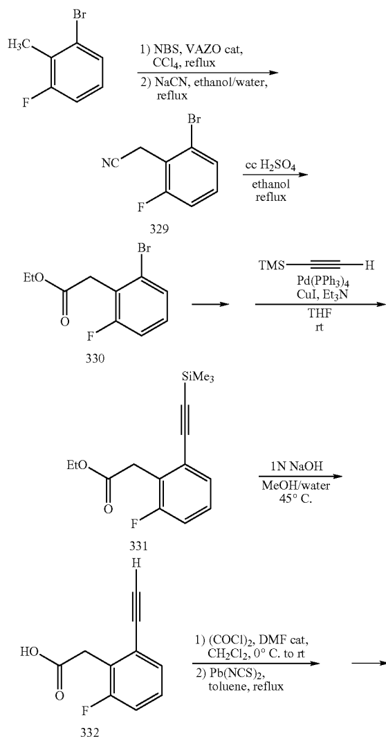
Scheme 77
