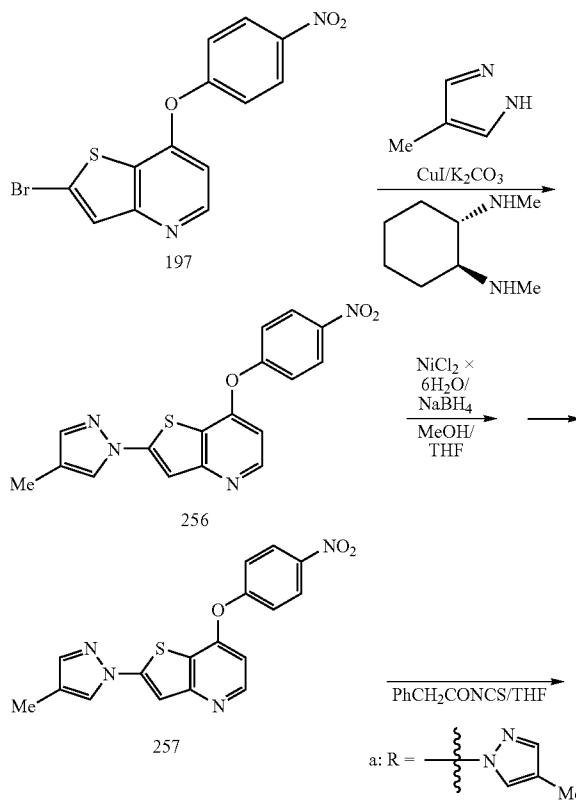
Scheme 58
