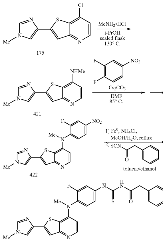
Scheme 85
