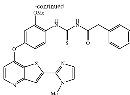
217: Example 193
