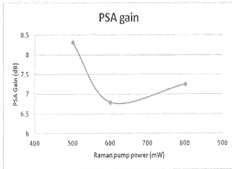
500 OPTICAL AMPLIFIER GAIN VERSUS RAMAN PUMP POWER
