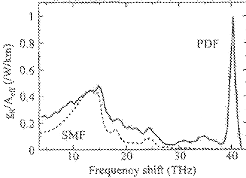
Fig. 1 Raman gain profiles of PDF and SMF
