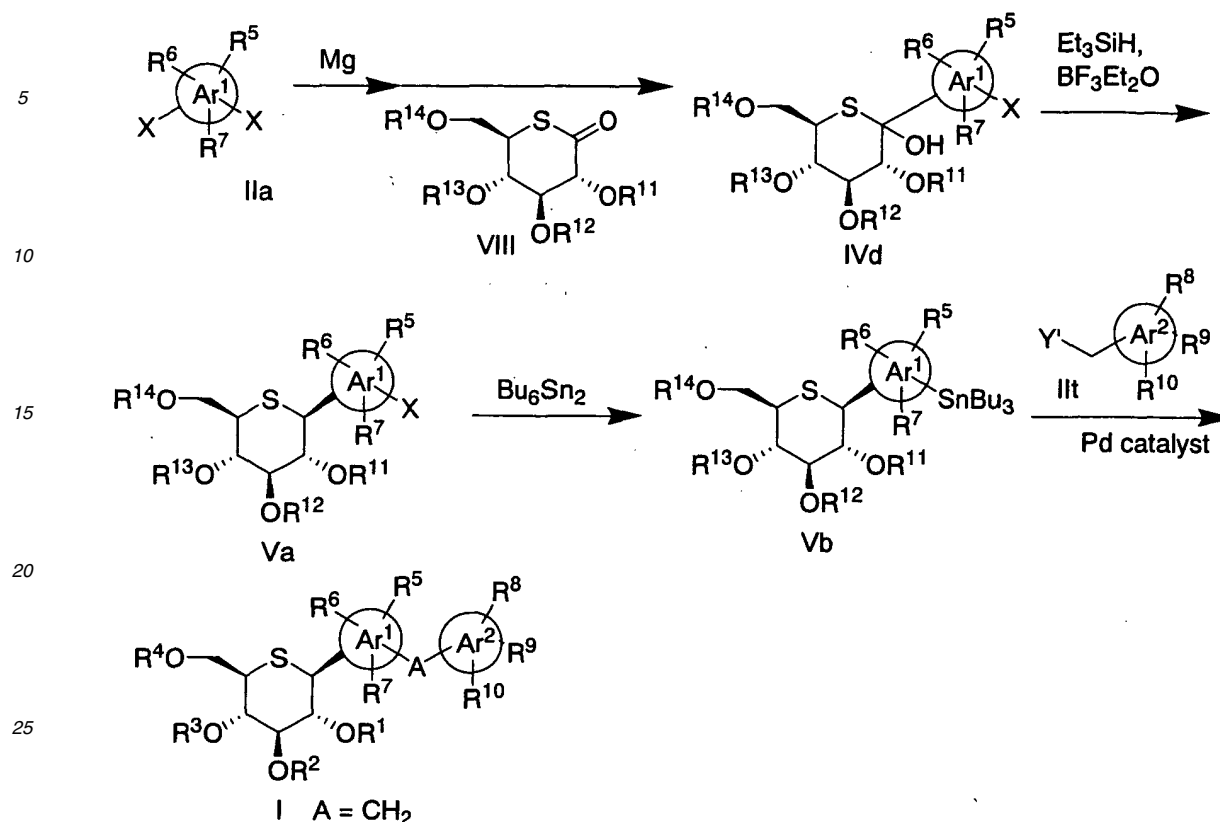
Scheme 12
