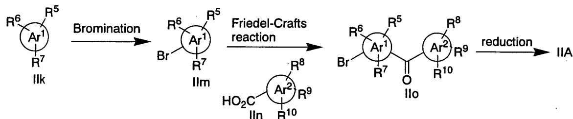
Scheme 8
