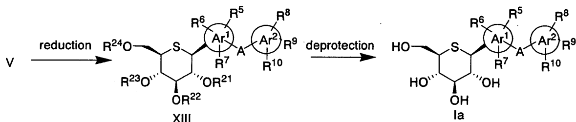
Scheme 4
