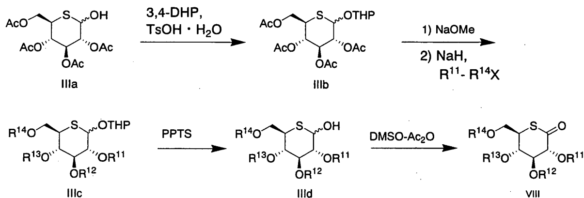
Scheme 9
