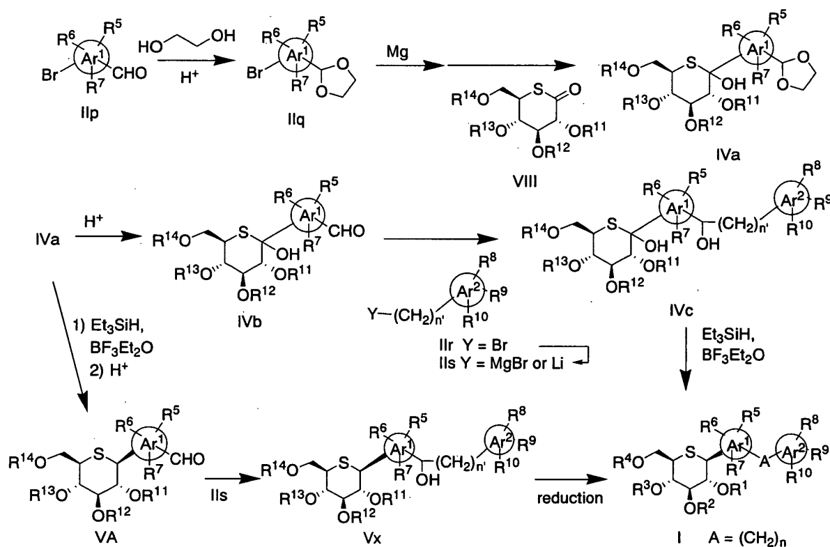
Scheme 10
