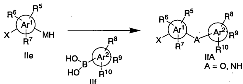
Scheme 6
