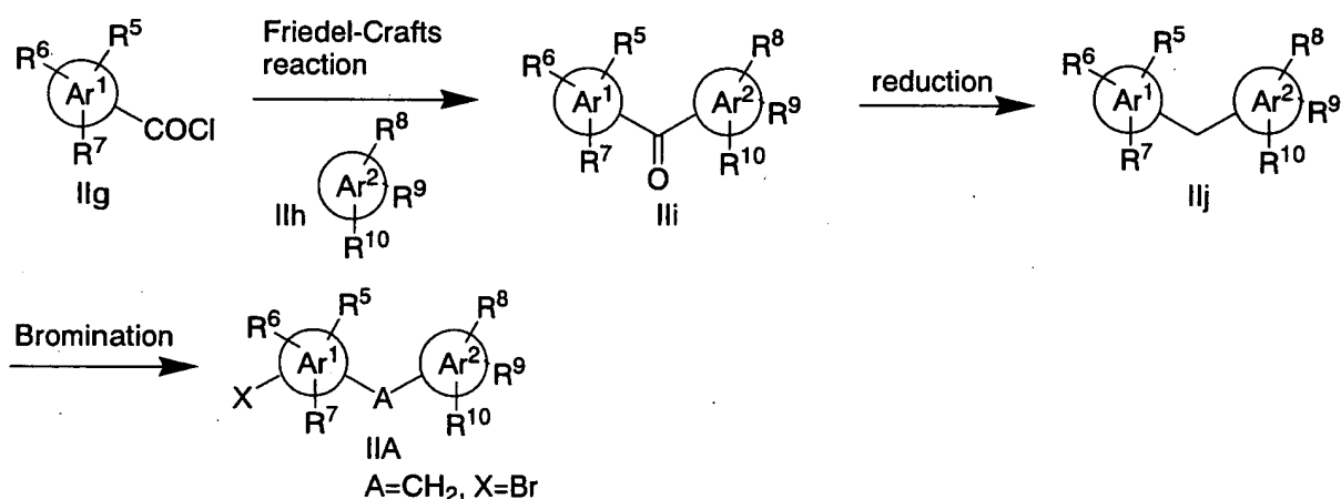
Scheme 7
