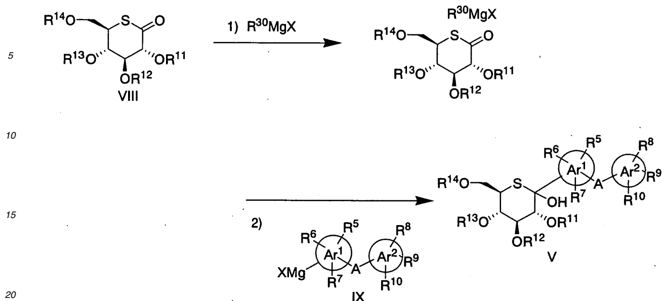
Scheme 3
