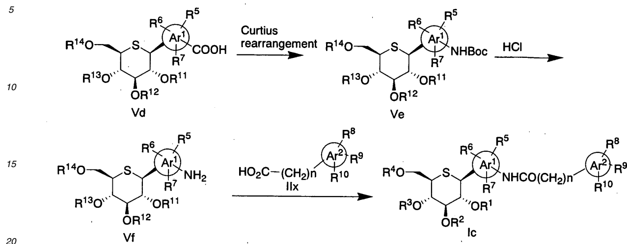
Scheme 16
