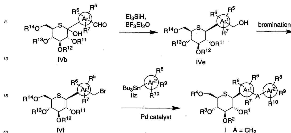
Scheme 13
