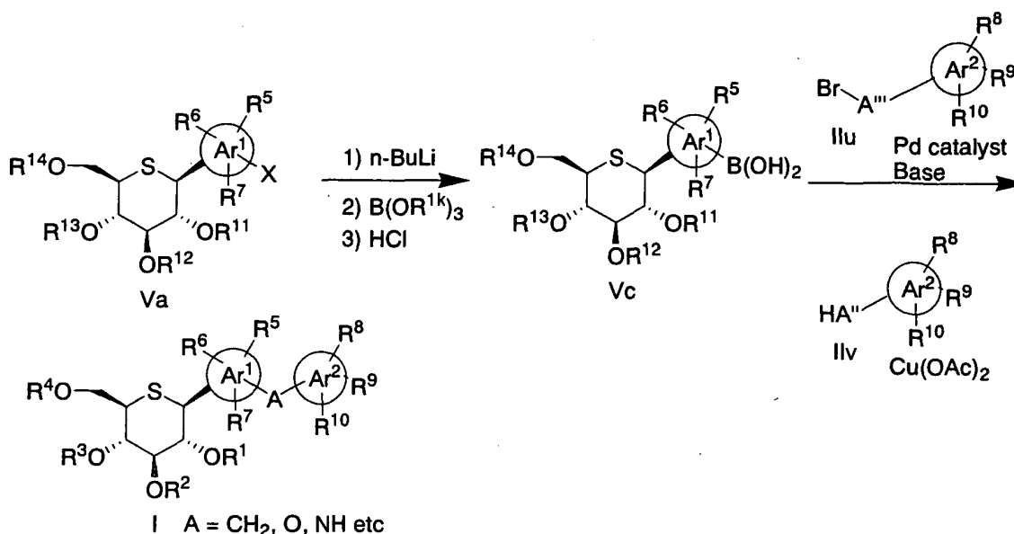
Scheme 14
