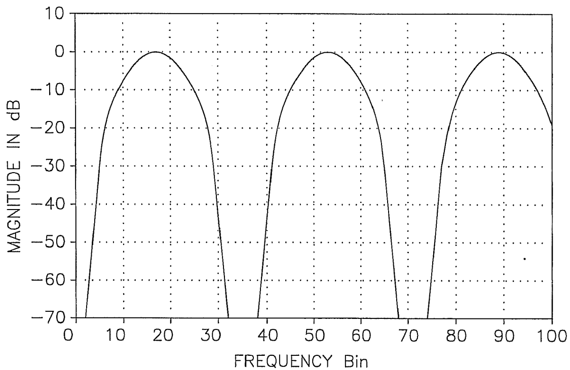
Magnitude response of a single polyphase filter bank
