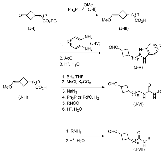
Scheme J: Elaboration of Cyclobutane
