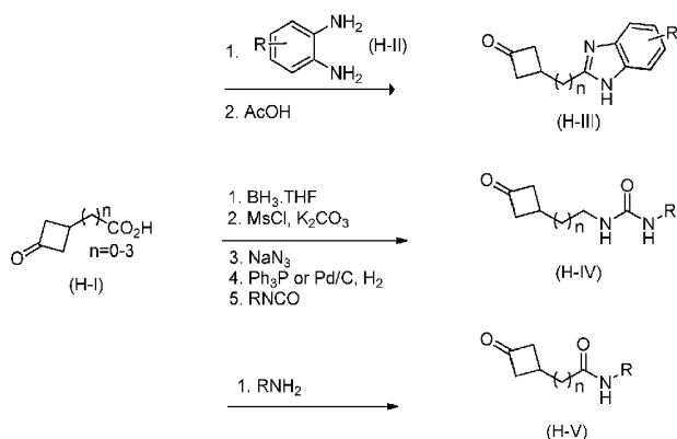
Scheme H: Elaboration of Cyclobutanones
