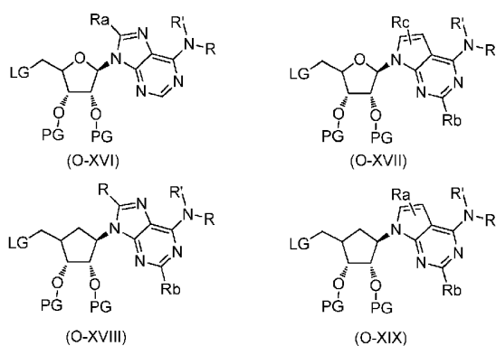
Scheme P: Amine, Amide and Sulfonamide Caps
