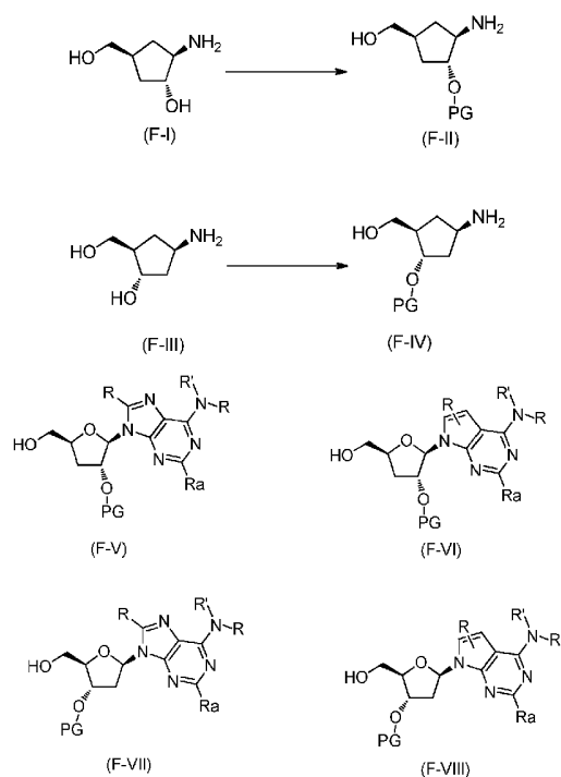
Scheme F: 2' and 3' Deoxycyclopentanes and Riboses
