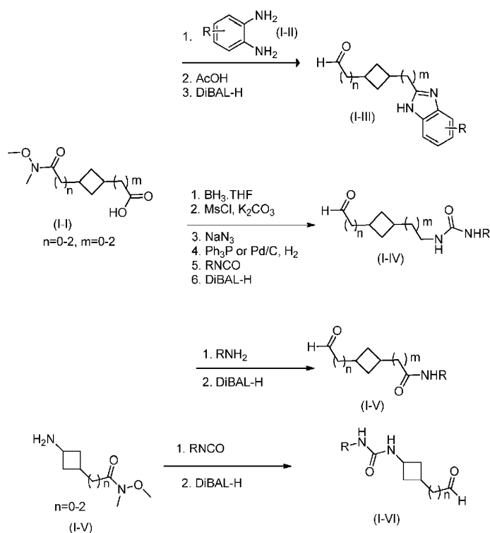
Scheme I: Elaboration of Cyclobutane Weinreb Amides
