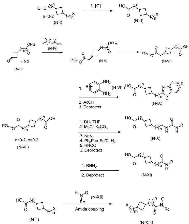
Scheme N: Synthesis of Amides
