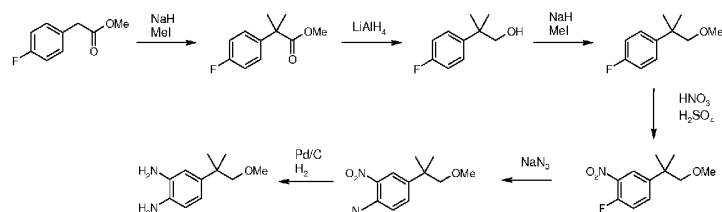
Scheme Q: Preparation of 4-(1-methoxy-2-methylpropan-2-yl)benzene-1,2-diamine
