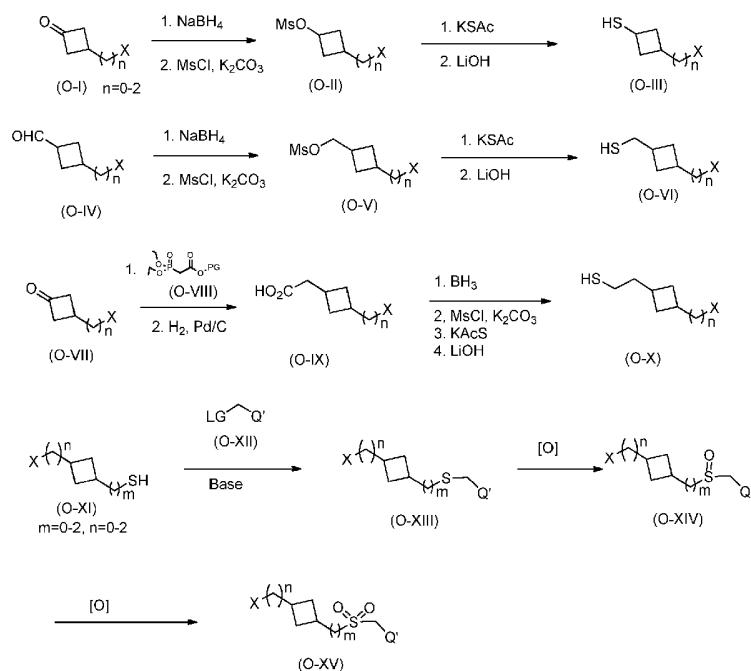
Scheme O: 5'-Sulfur Containing Analogs
