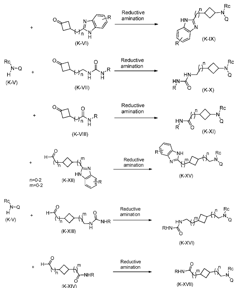
Scheme K: Coupling of Cyclobutanes to Amines
