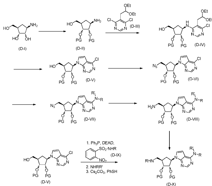
Scheme D: 7-Deazapurine-carbocyclic Intermediates Synthesis
