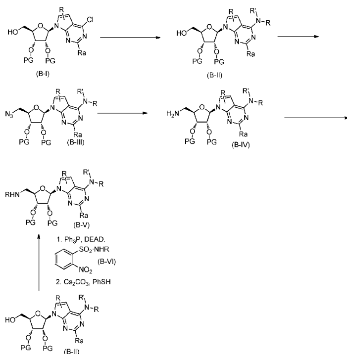
Scheme B: 5' Amino 7-Deazapurine Ribose Synthesis
