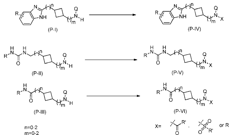
Scheme P: Amine, Amide and Sulfonamide Caps
