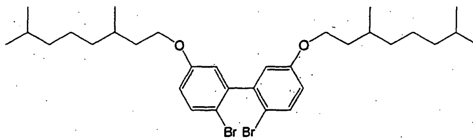
Compound E
