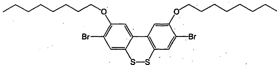
Compound B
