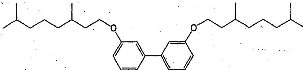
Compound D
