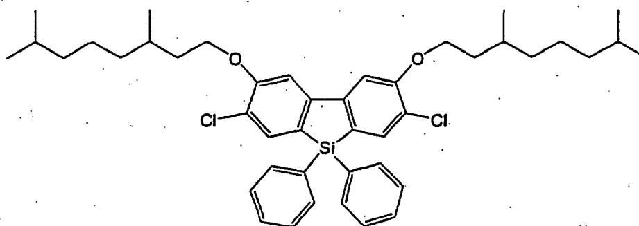
Compound H
