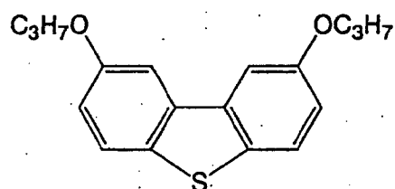
Calculation compound 1
