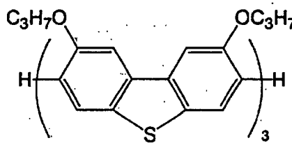
Calculation compound 2
