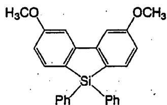
Calculation compound 5
