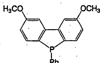
Calculation compound 6
