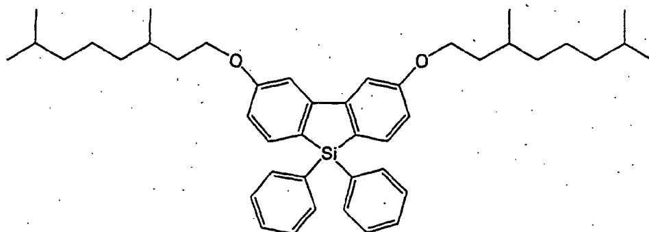
Compound F
