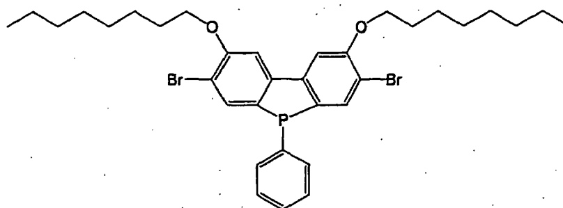
Compound A
