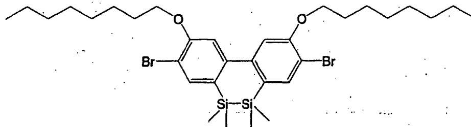
Compound C
