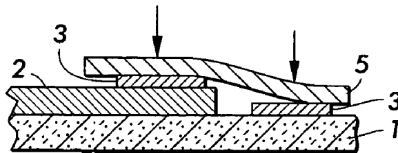
FIG. 2 PRIOR ART
