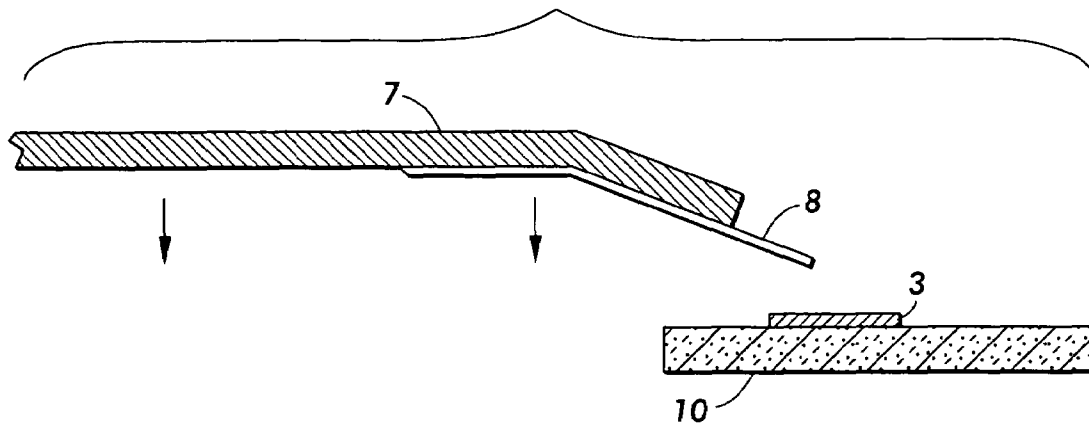
FIG. 5 PRIOR ART
