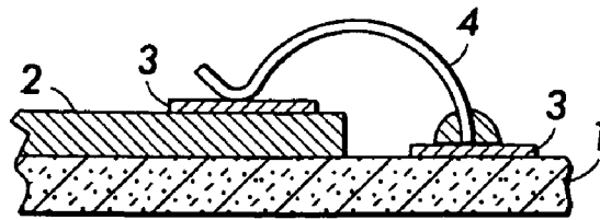
FIG. 1 PRIOR ART
