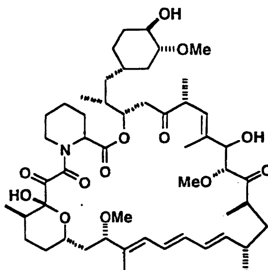
Rapamycin
