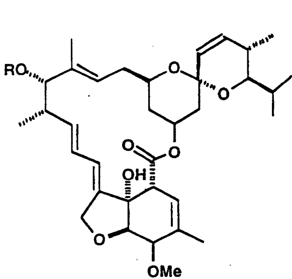
Avermectin A1b
