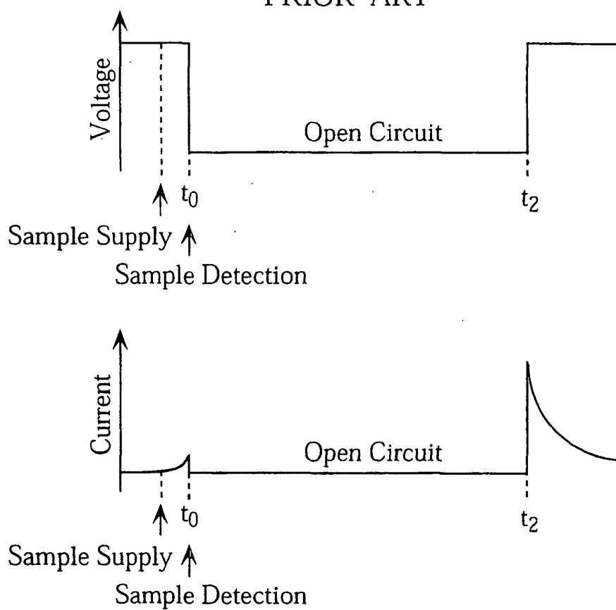
FIG.10 PRIOR ART
