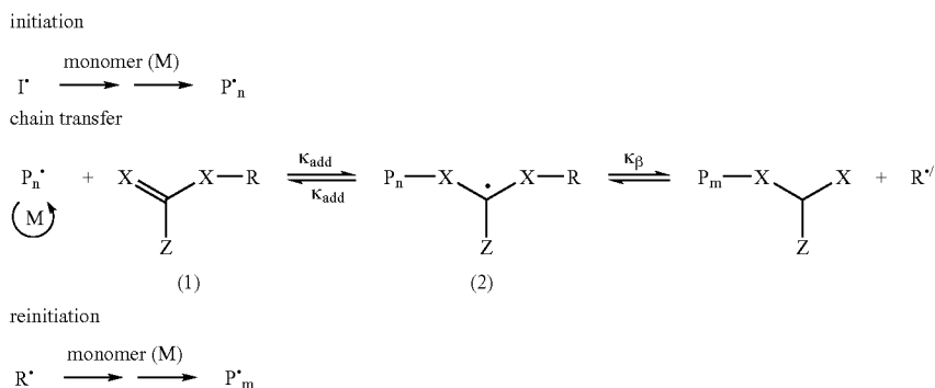
Scheme 1. Proposed mechanism of RAFT polymerisation
