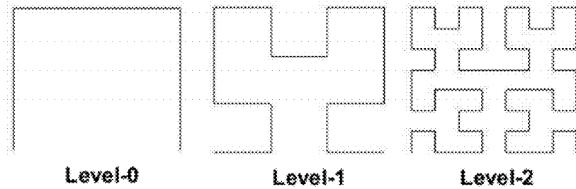
FIGURE 6(b): Hilbert Curve generated up to 3 levels
