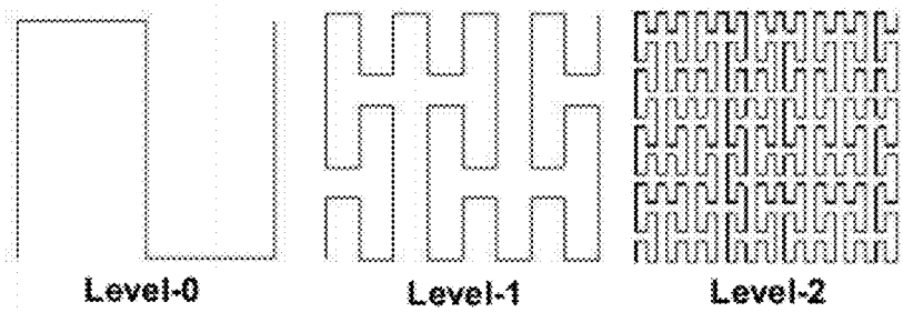
FIGURE 6(a): Peano curve generated up to 3 levels
