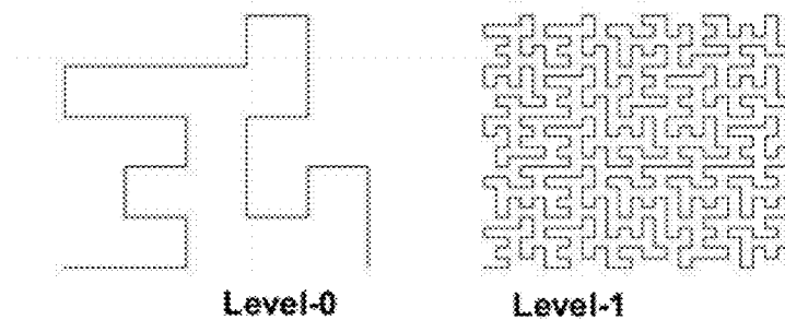
FIGURE 6(d): E-curve curve generated up to 2 levels
