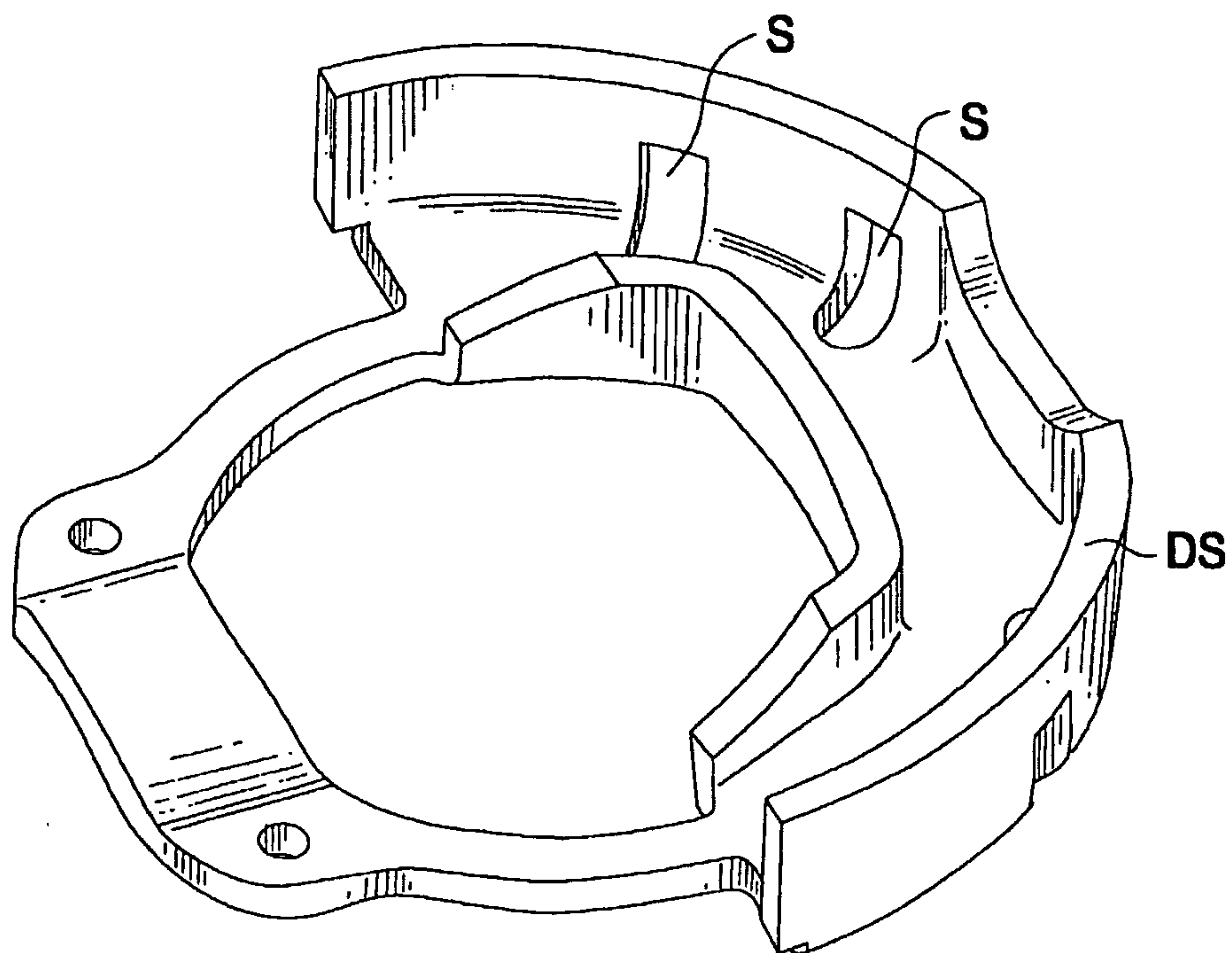
FIG. 8 PRIOR ART
