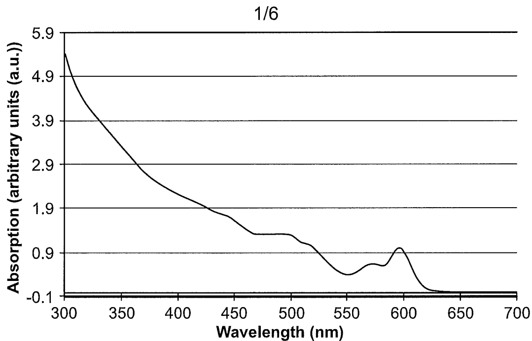
Absorption spectrum of the CdSe core of Example III (596nm peak, 12nm HWHM).
