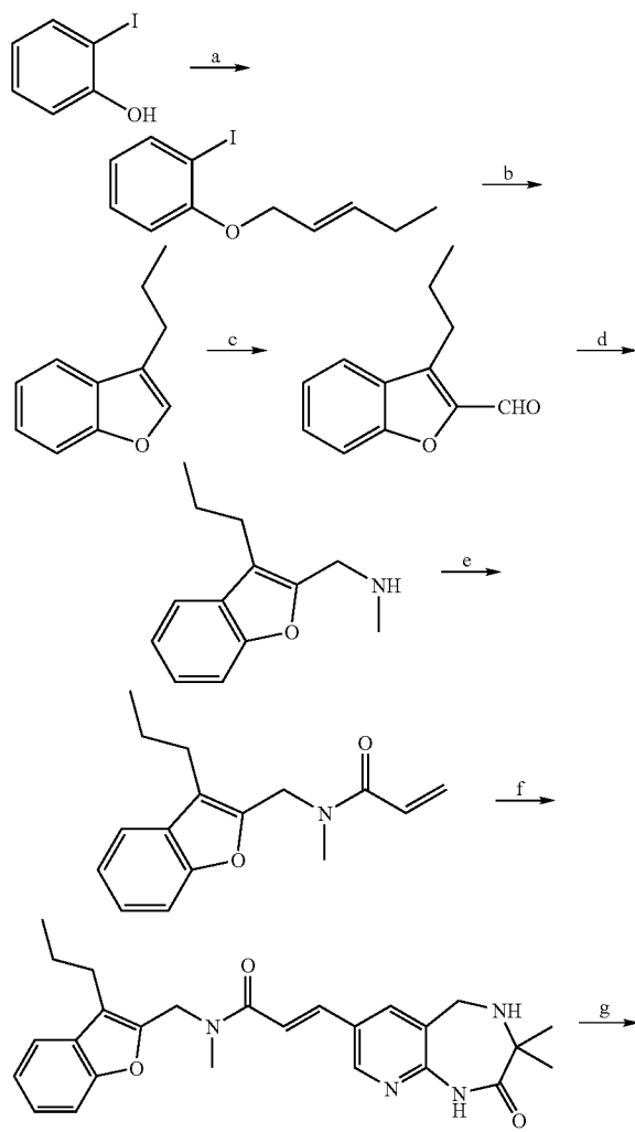
Scheme 12.
