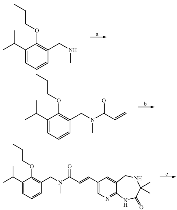
Scheme 5.
