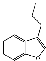
C_{11}H_{12}O Exact Mass: 160.09
