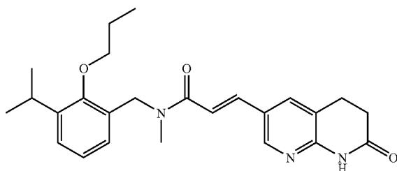
\text{C}_{25}\text{H}_{31}\text{N}_3\text{O}_3 Exact Mass: 421.24
