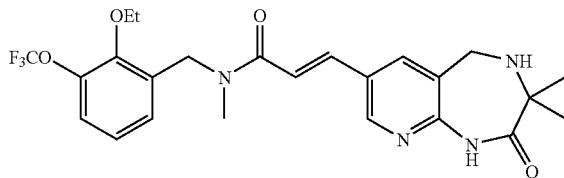
C_{24}H_{27}F_3N_4O_4 Exact Mass: 492.20
