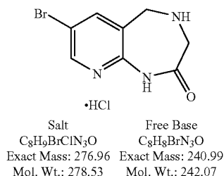
a) 7-Bromo-1,3,4,5-tetrahydropyrido[2,3-e][1,4]diazepin-2-one hydrochloride
