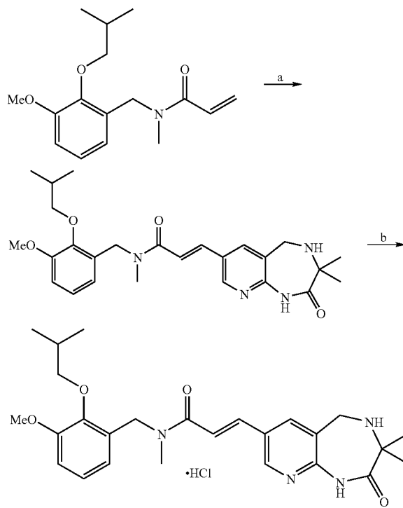
Scheme 8.
