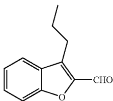
C_{12}H_{12}O_2 Exact Mass: 188.08
