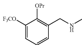
\text{C}_{12}\text{H}_{16}\text{F}_3\text{NO}_2 Exact Mass: 263.11
