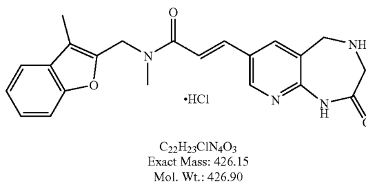
c) (E)-N-Methyl-N-(3-methylbenzofuran-2-ylmethyl)-3-(2-oxo-2,3,4,5-tetrahydro-1H-pyrido[2,3-e][1,4]diazepin-7-yl)acrylamide hydrochloride
