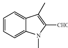
b) 1,3-dimethyl-1H indole-2-carbaldehyde
