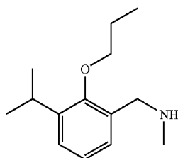
\text{C}_{14}\text{H}_{23}\text{NO} Exact Mass: 221.18
