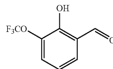
C_8H_5F_3O_3 Exact Mass: 206.02
