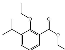
\text{C}_{14}\text{H}_{20}\text{O}_3 Exact Mass: 236.14
