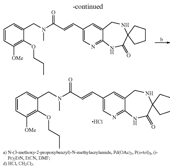
Scheme 12.
