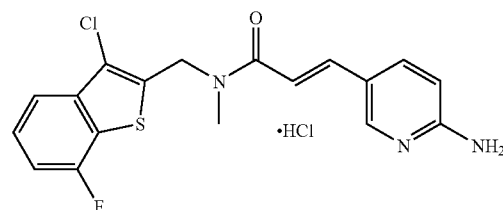
Free Base HCl Salt \text{C}_{18}\text{H}_{15}\text{ClFN}_3\text{OS} \text{C}_{18}\text{H}_{16}\text{Cl}_2\text{FN}_3\text{OS} Exact Mass: 375.06 Exact Mass: 411.04
