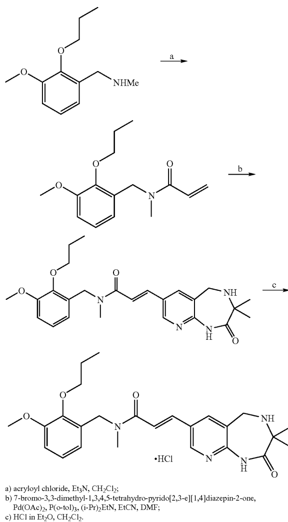
Scheme 15.
