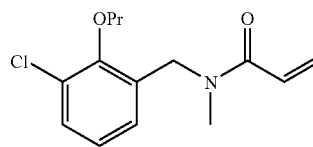
C 14 H 18 ClNO 2 Exact Mass: 267.10
