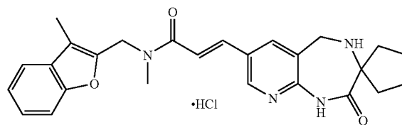
C 26 H 29 ClN 4 O 3 Exact Mass: 480.19
