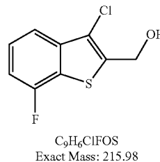
b) (3-chloro-7-fluoro-benzo[b]thiophen-2-yl)methanol
