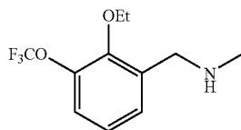
C_{11}H_{14}F_3NO_2 Exact Mass: 249.10
