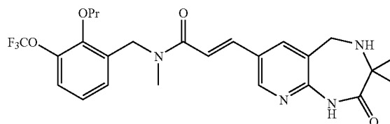
\text{C}_{25}\text{H}_{29}\text{F}_3\text{N}_4\text{O}_4 Exact Mass: 506.21
