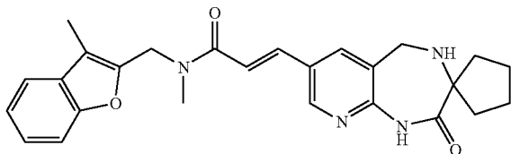
C 26 H 28 N 4 O 3 Exact Mass: 444.22
