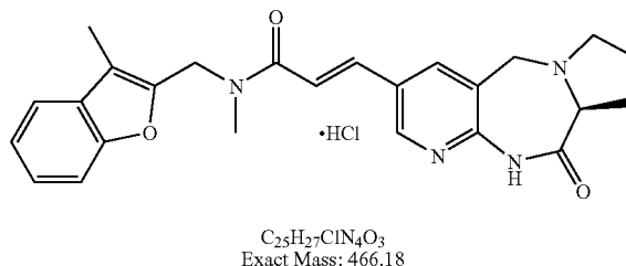
b) (S)-(+)-(E)-N-Methyl-N-(3-methylbenzofuran-2-ylmethyl)-3-(10-oxo-2,3,4,9,10,10a-hexahydro-1H-3a,8,9-triazabenzof[f]azulen-6-yl)acrylamide hydrochloride
