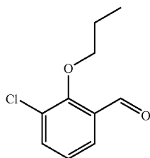
C 10 H 11 ClO 2 Exact Mass: 198.04
