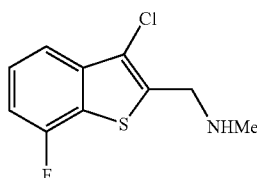
\text{C}_{10}\text{H}_6\text{ClFNS} Exact Mass: 229.01
