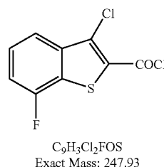
a) 3-chloro-7-fluoro-benzo[b]thiophene-2-carbonyl chloride
