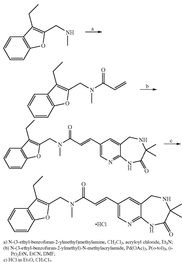
Scheme 13.
