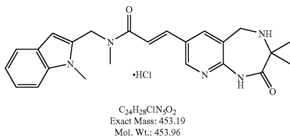
c) (E)-3-(3,3-Dimethyl-2-oxo-2,3,4,5-tetrahydro-1H-pyrido[2,3-e][1,4]diazepin-7-yl)-N-methyl-N-(1-methyl-1H-indol-2-ylmethyl)acrylamide hydrochloride
