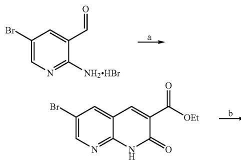
Scheme 9.
