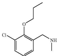
C 11 H 16 ClNO Exact Mass: 213.09
