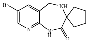
C 12 H 14 BrN 3 O Exact Mass: 295.03
