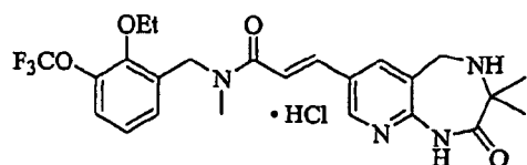
Figure 3a.
