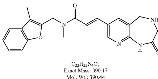
b) (E)-N-Methyl-N-(3-methylbenzofuran-2-ylmethyl)-3-(2-oxo-2,3,4,5-tetrahydro-1H-pyrido[2,3-e][1,4]diazepin-7-yl)acrylamide
