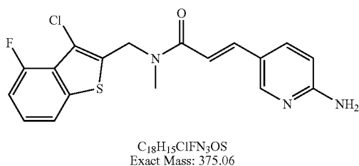
e) (E)-3-(6-amino-pyridin-3-yl)-N-(3-chloro-4-fluoro-benzo[b]thiophen-2-ylmethyl)-N-methylacrylamide
