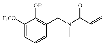
C_{14}H_{16}F_3NO_3 Exact Mass: 303.11
