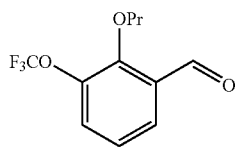
\text{C}_{11}\text{H}_{11}\text{F}_3\text{O}_3 Exact Mass: 248.07
