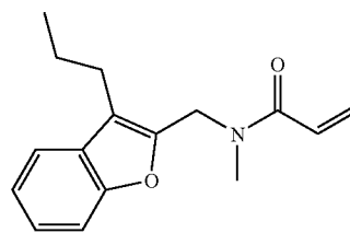
C_{16}H_{19}NO_2 Exact Mass: 257.14
