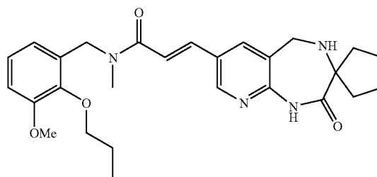
C 27 H 34 N 4 O 4 Exact Mass: 478.26
