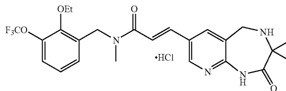
C_{24}H_{28}ClF_3N_4O_4 Exact Mass: 528.18
