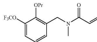
\text{C}_{15}\text{H}_{18}\text{F}_3\text{NO}_3 Exact Mass: 317.12
