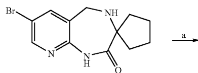
Scheme 11.
