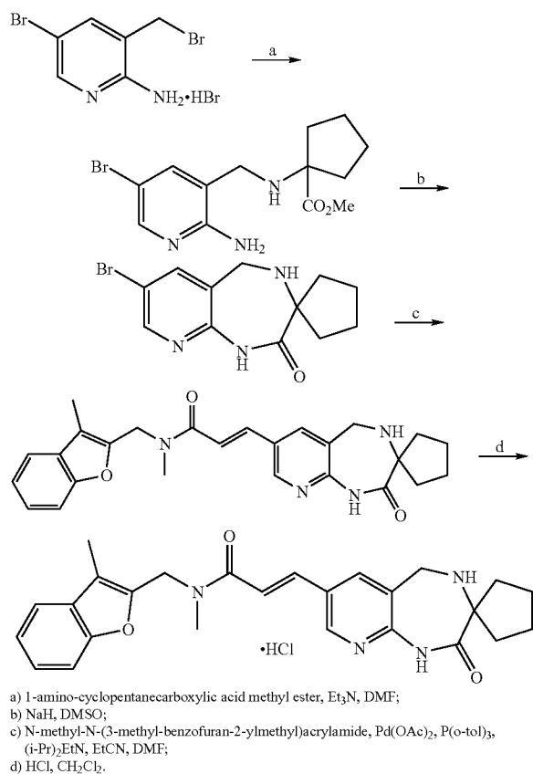
Scheme 10.
