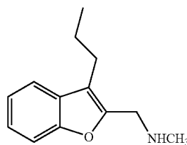
C_{13}H_{17}NO Exact Mass: 203.13
