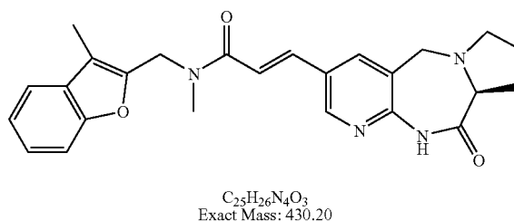
a) (S)-(+)-(E)-N-Methyl-N-(3-methylbenzofuran-2-ylmethyl)-3-(10-oxo-2,3,4,9,10,10a-hexahydro-1H-3a,8,9-triazabenzof[f]azulen-6-yl)acrylamide
