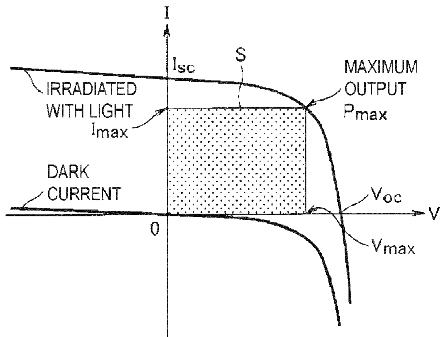
CURRENT-VOLTAGE CHARACTERISTICS OF SOLAR CELL
