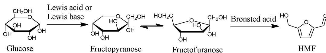
Reaction Scheme 1
