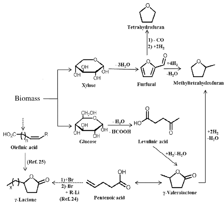
Reaction Scheme 2
