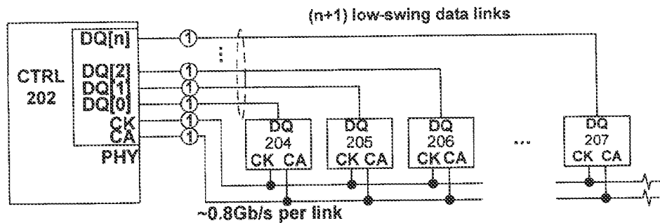
Large-swing (CMOS/PODL) command/address link and clock link
