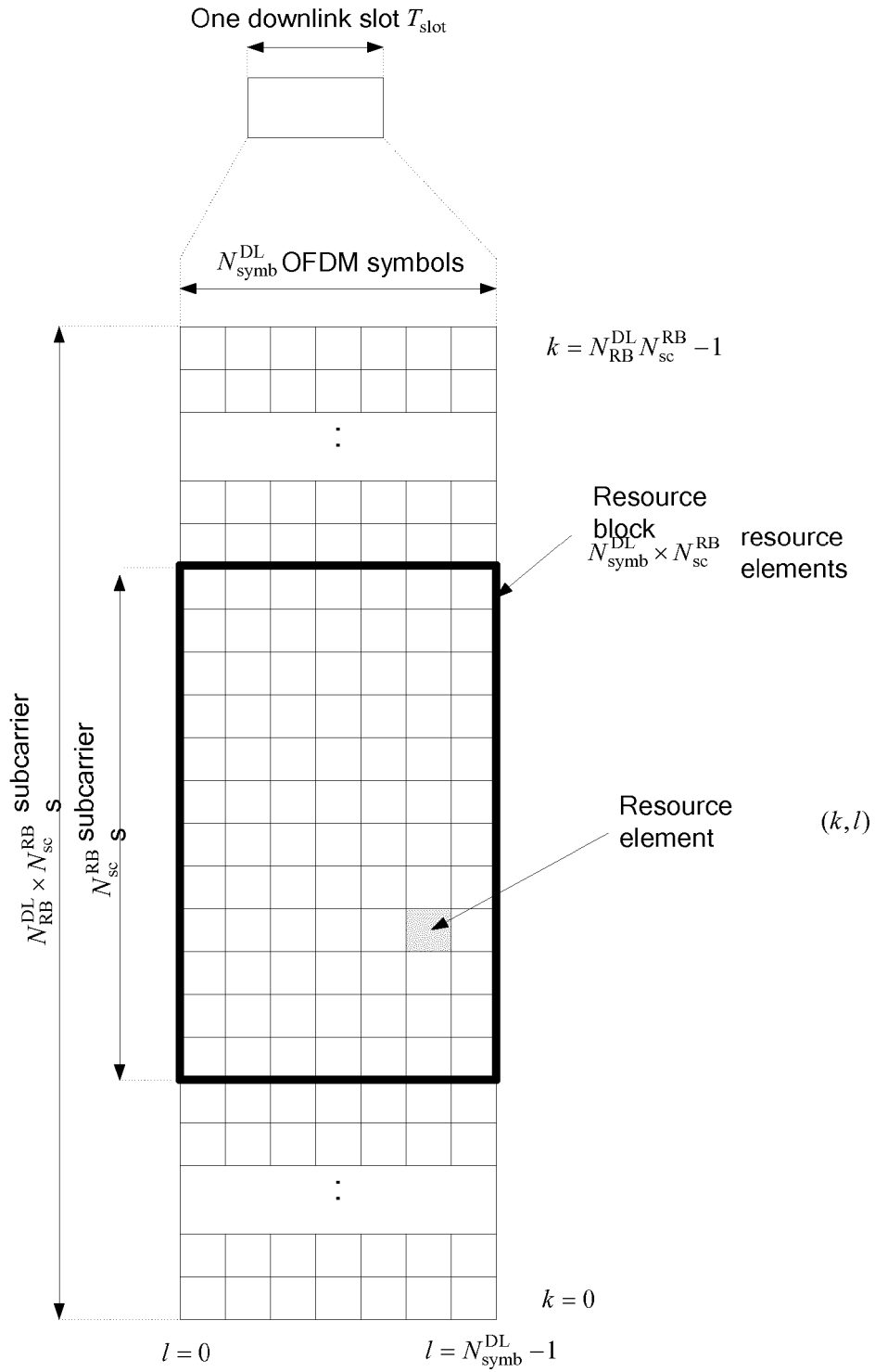
FIG. 10 (PRIOR ART)
