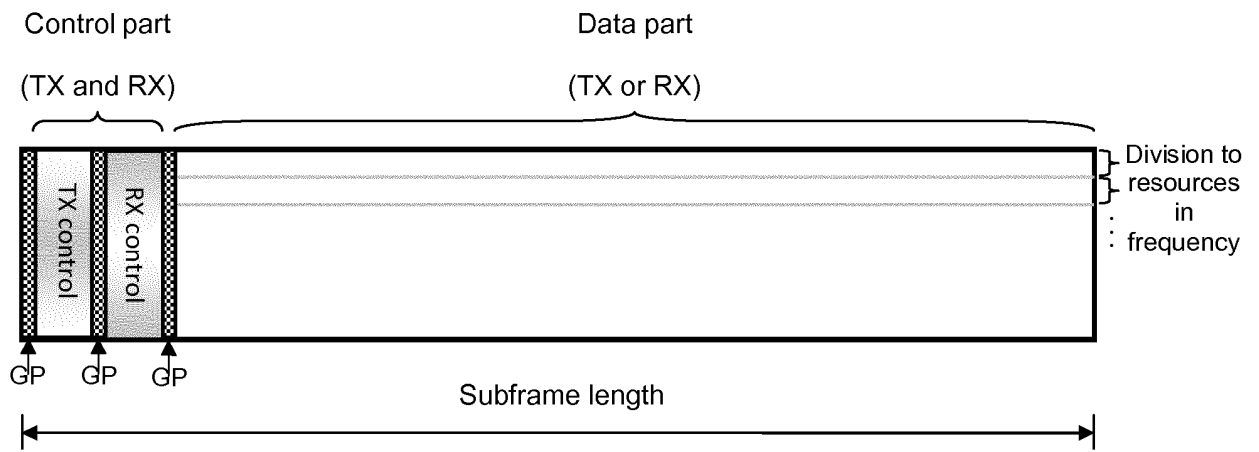
FIG. 12 (PRIOR ART)
