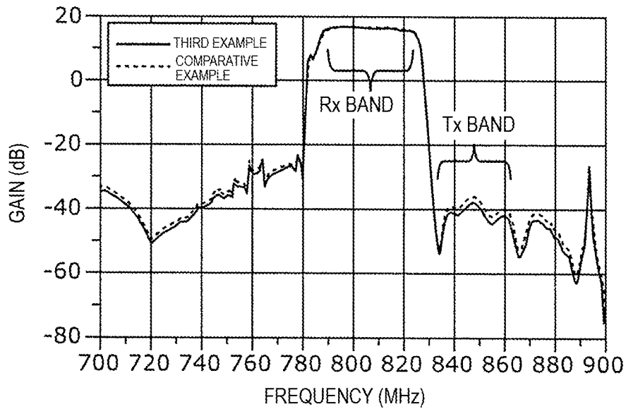
DupRx-LNA TRANSMISSION CHARACTERISTICS
