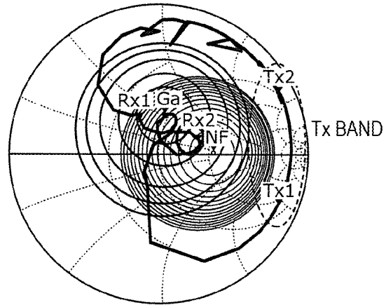
THIRD EXAMPLE DUPLEXER Rx IN-BAND IMPEDANCE: 110Ω
