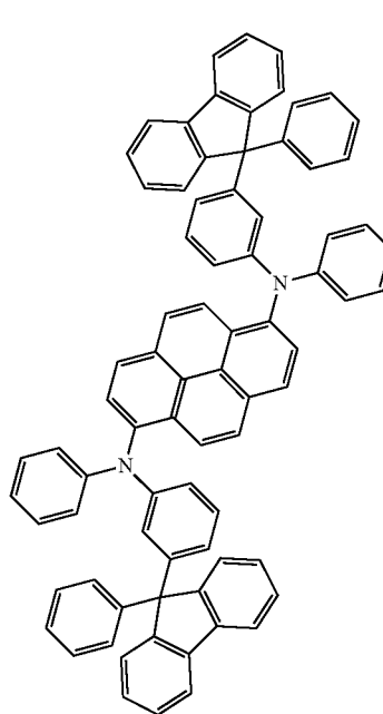
Step 1: Synthesis method of 9-(3-bromophenyl)-9-phenylfluorene
