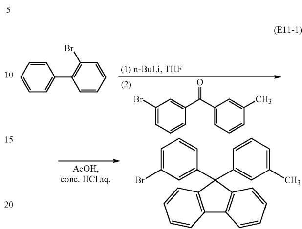
Step 2: Synthesis method of 3-[9-(3-methylphenyl)-9H-fluoren-9-yl]diphenylamine (abbreviation: mFLPA-II)
