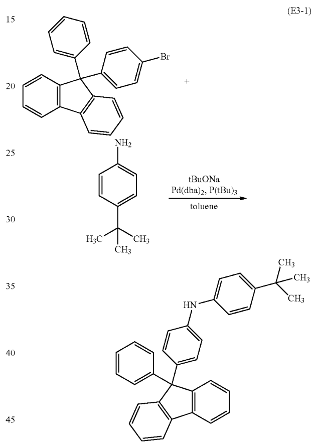
Step 2: Synthesis example of N,N'-bis[4-(9-phenyl-9H-fluoren-9-yl)phenyl]-N,N'-bis(4-tert-butylphenyl)-pyrene-1,6-diamine (abbreviation: 1,6tBu-FLPAPrn)
