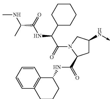
A 410099.1 amine
