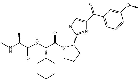
LCL 161, hydroxyl
