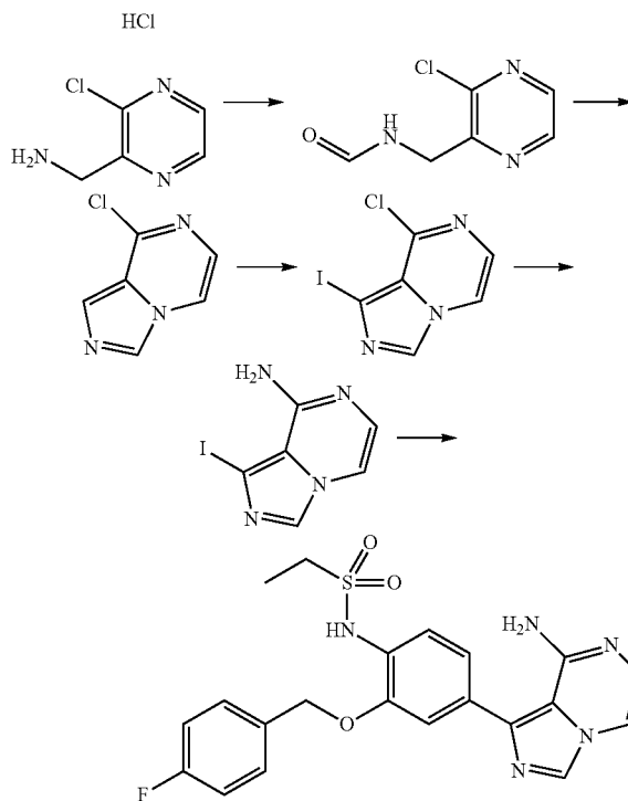
Step 1: N-((3-Chloropyrazin-2-yl)methyl)formamide
