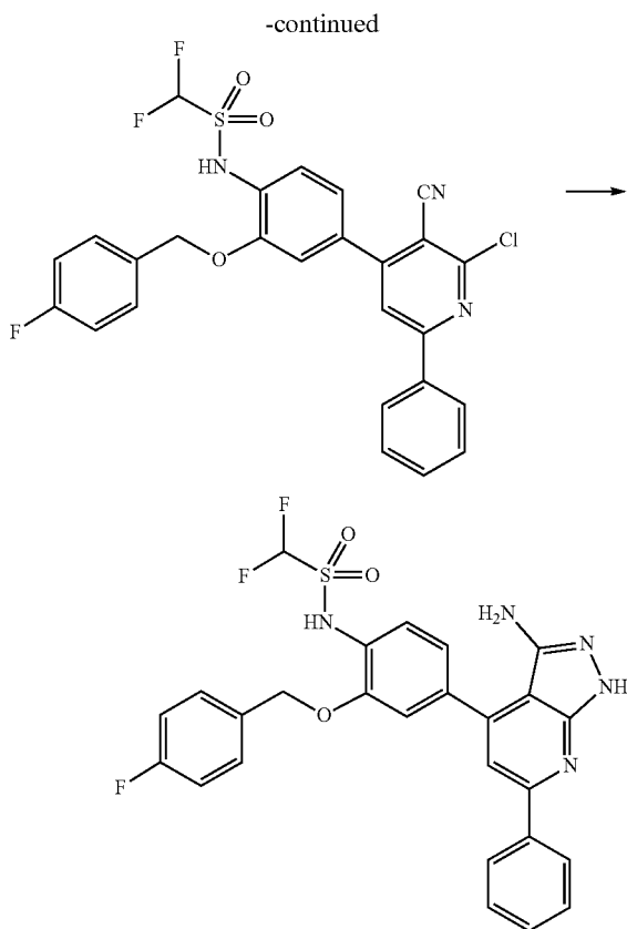
Step 1: 4-(3-((4-Fluorophenyl)methoxy)-4-nitrophenyl)-2-oxo-6-phenyl-1,2-dihydropyridine-3-carbonitrile
