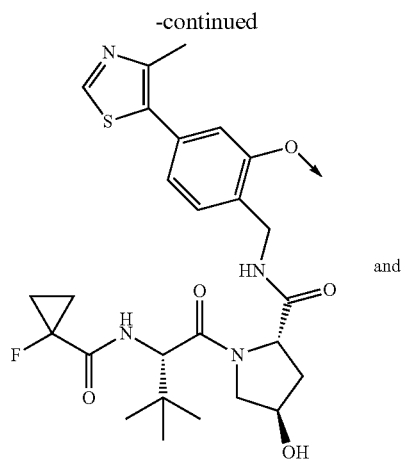
VH 101, phenol
