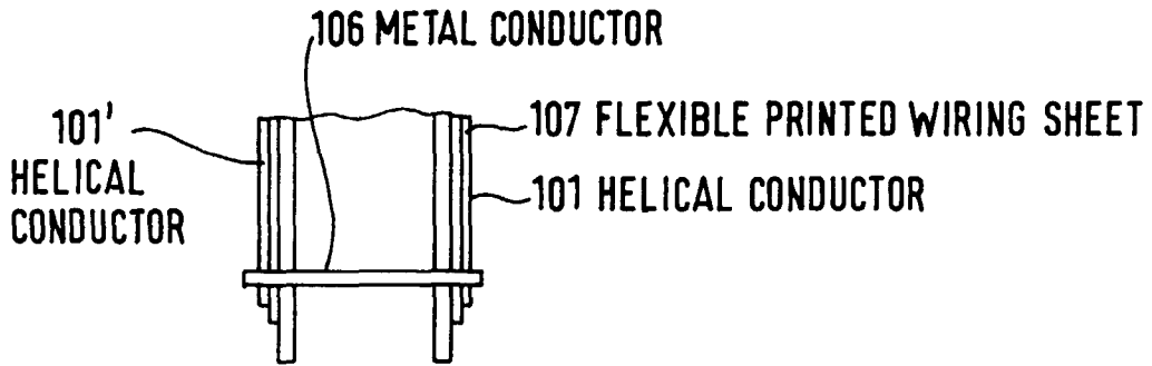
FIG. 9 (Prior Art)
