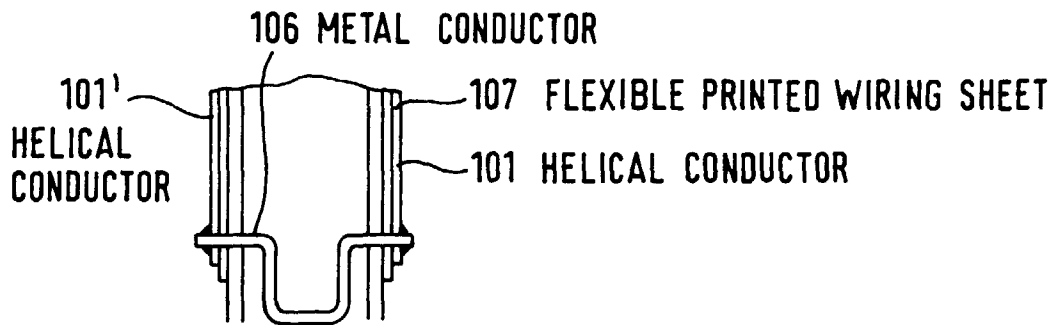
FIG. 10 (Prior Art)
