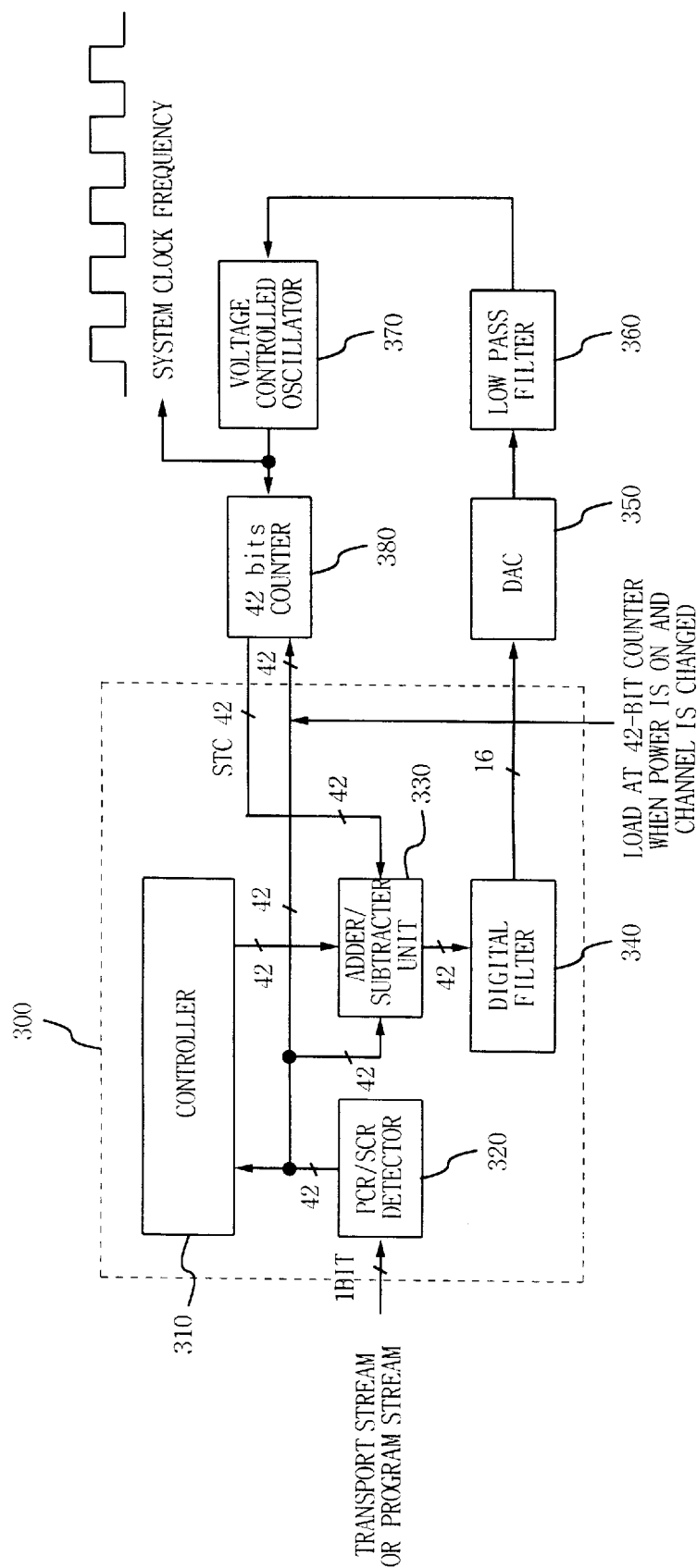
FIG. 3(PRIOR ART)
