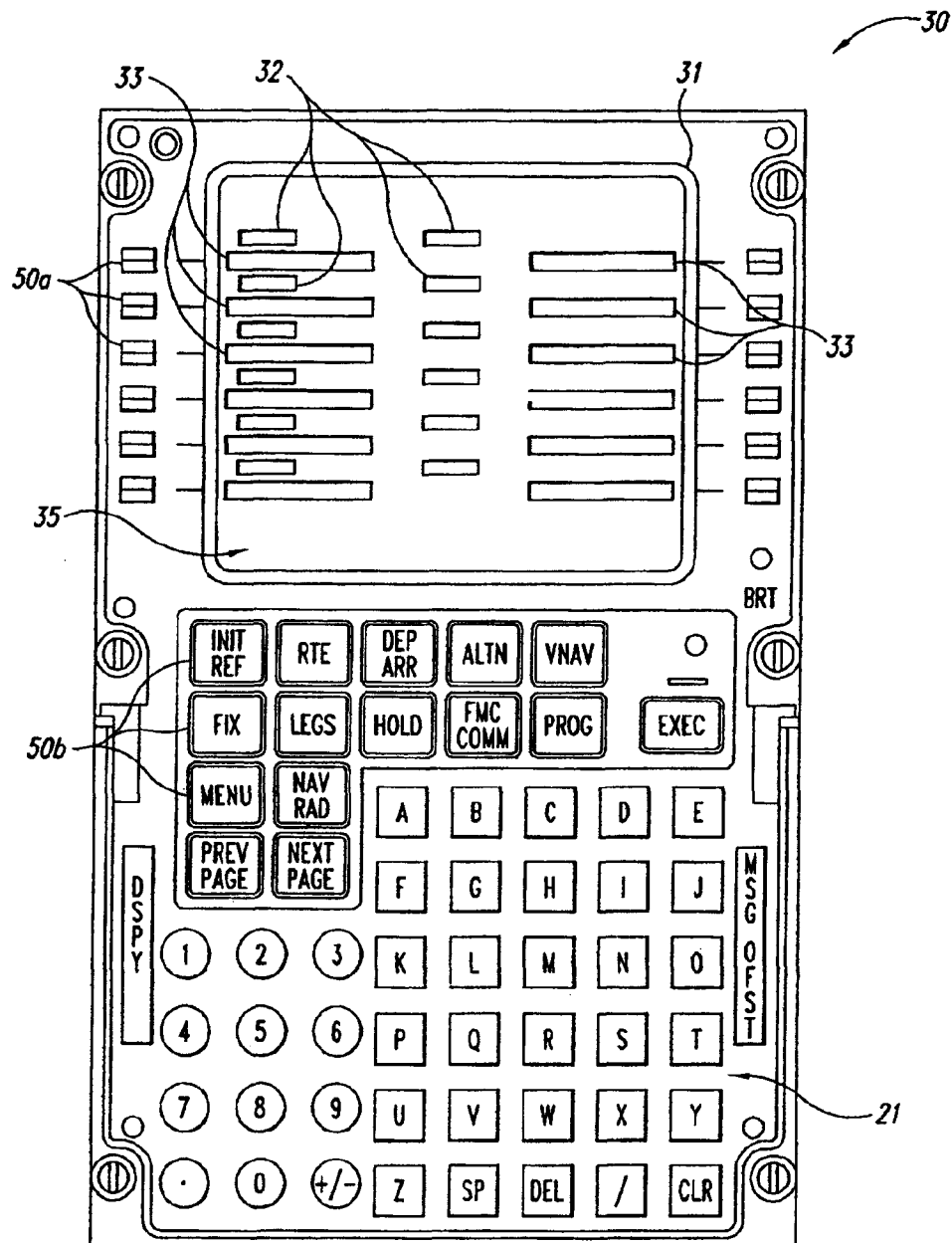
Fig. 1 (Prior Art)
