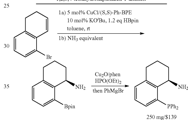
Scheme 3-2. Preparation of (R)-8-(diphenylphosphino)-1,2,3,4-tetrahydronaphthalen-1-amine.
