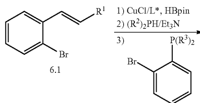
Scheme 6. Trans-spanning ligands.
