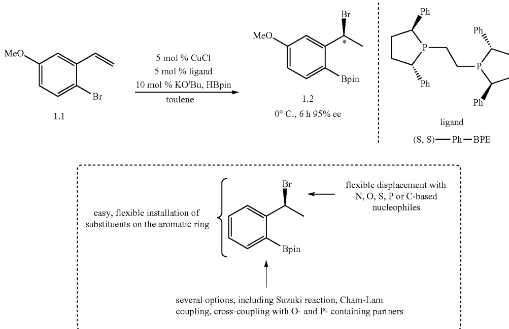
Scheme 1.1 Enantioselective Cu-catalyzed halogenation.
