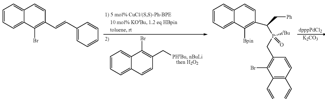
Scheme 3-3. Preparation of a dibenzyl binapine ligand.
