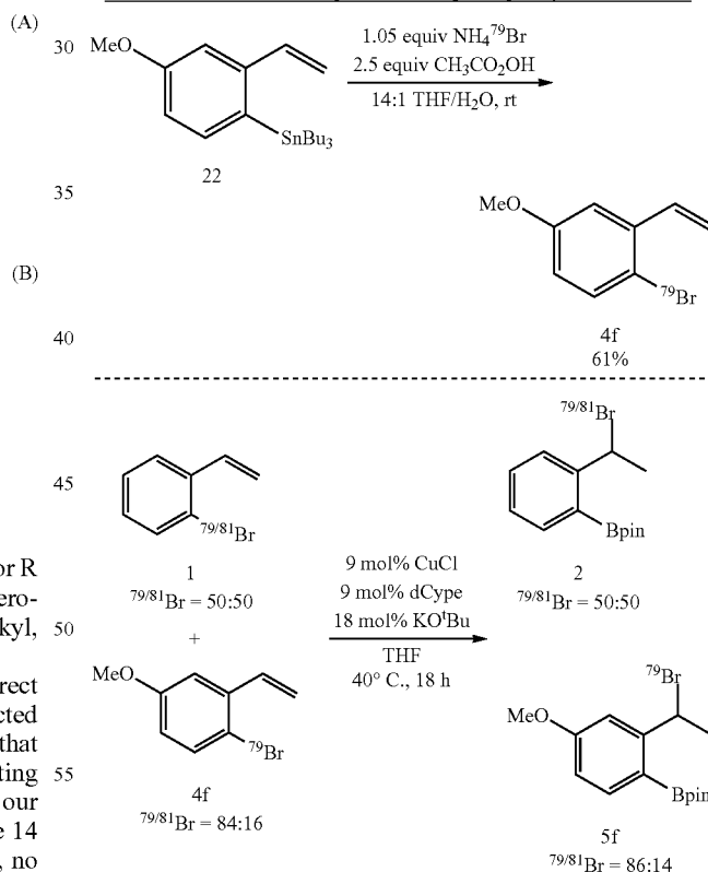
Scheme 1-3. Cross-Over Experiment Using Isotopically Enriched ^{79}Br . a
