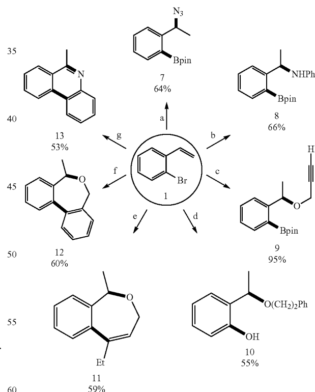
Scheme 1-2. Recycling of the Activating Group. a
