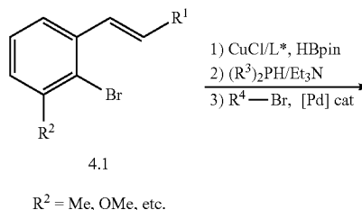
Scheme 4. New ligand classes with point and axial chirality.
