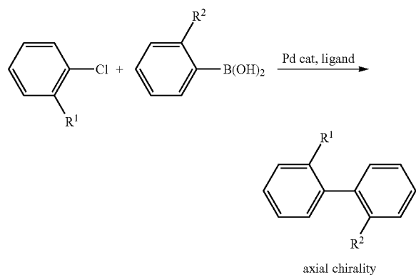
Scheme 7. Test reactions for novel ligands.
