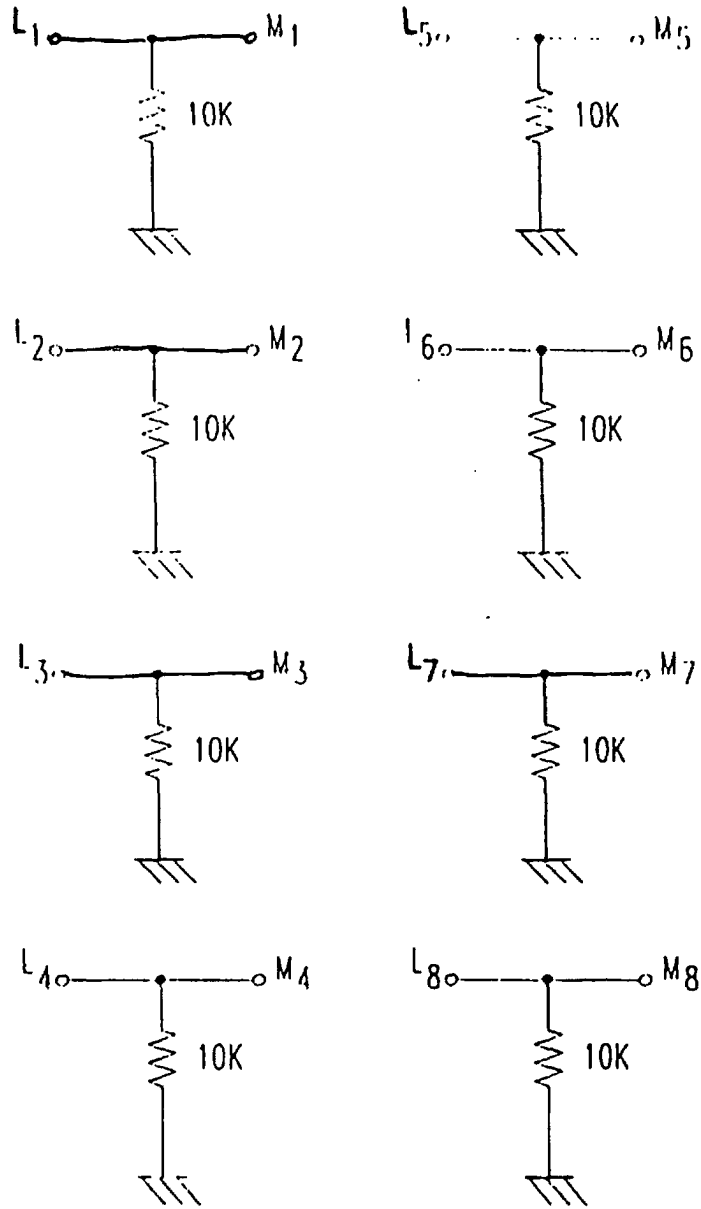
OUTPUT MUX LOAD RESISTORS
