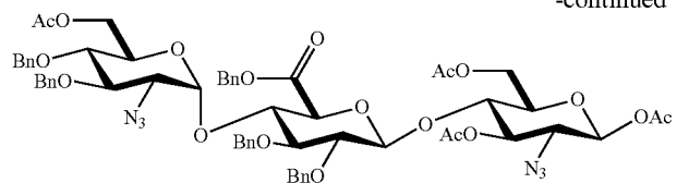
EDC-1-CB C_{59}H_{66}N_6O_{21} Mol. Wt.: 1195.18
