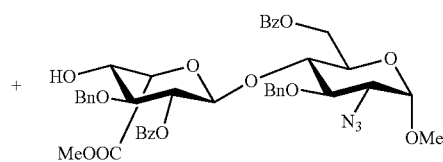
BA Dimer C_{42}H_{43}N_3O_{13} Mol. Wt.: 797.80
