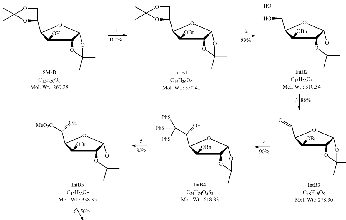
Scheme 2 - Synthesis of Monomer B-1 and BMod6 [Building Block B]
