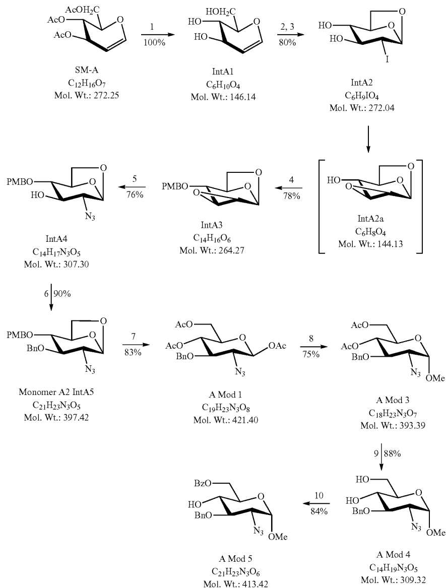
SCHEME 1 - Synthesis of Monomer A-2 &amp; AMod5 [Building Block A]
