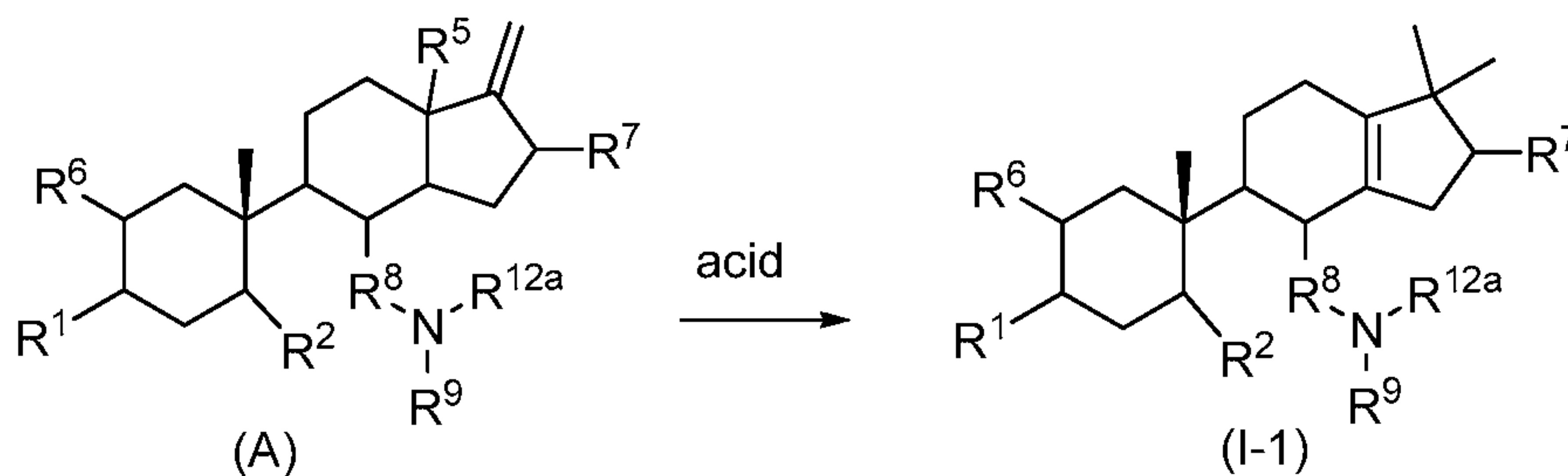
REACTION SCHEME 1A
