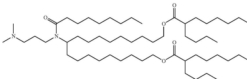
Compound II-17
