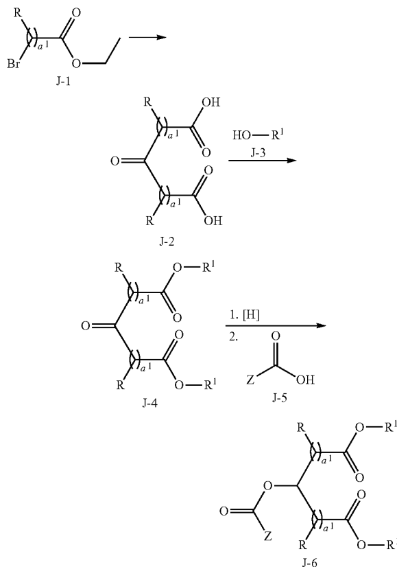
GENERAL REACTION SCHEME 10
