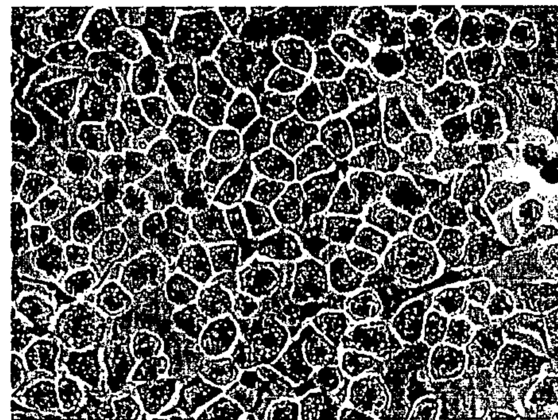
Adipogenesis G3.9
