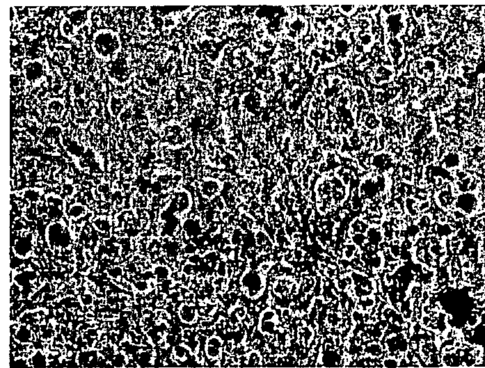
Osteogenesis G3.9
