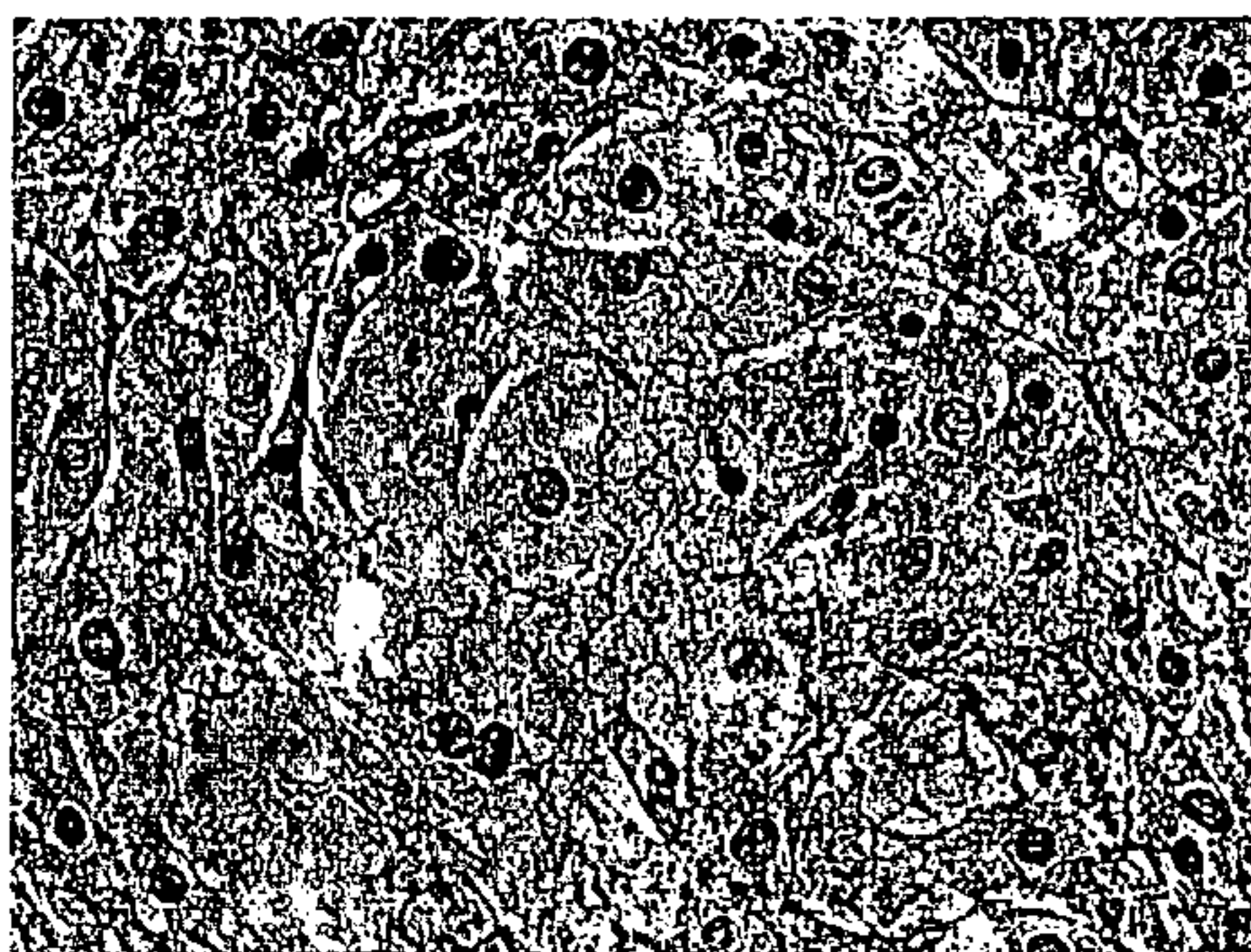
FIG. 9 Adipogenesis G3.8
