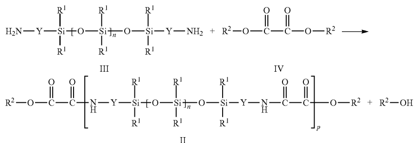
Reaction Scheme B
