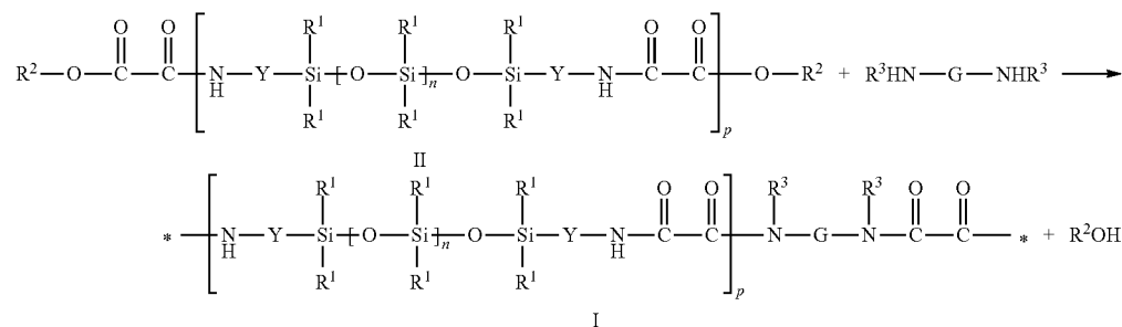
Reaction Scheme A
