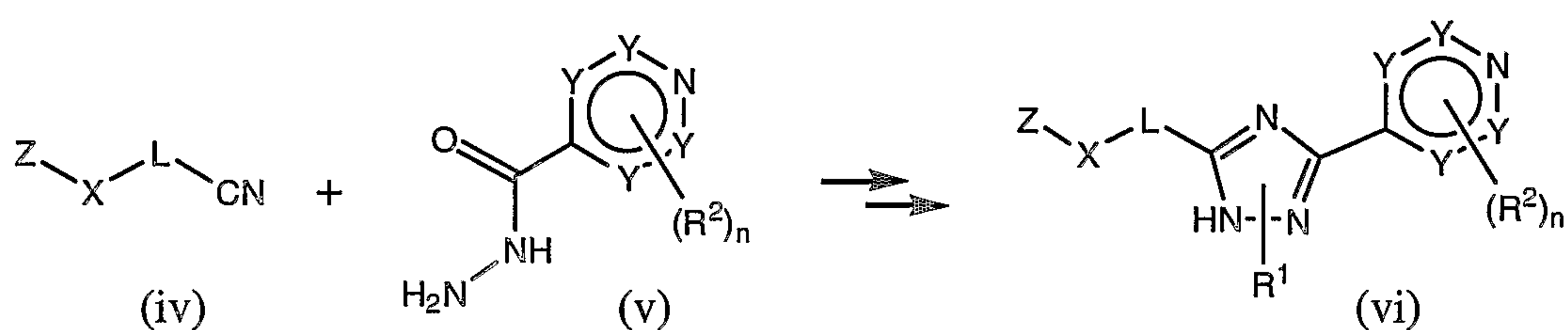
Scheme 2
