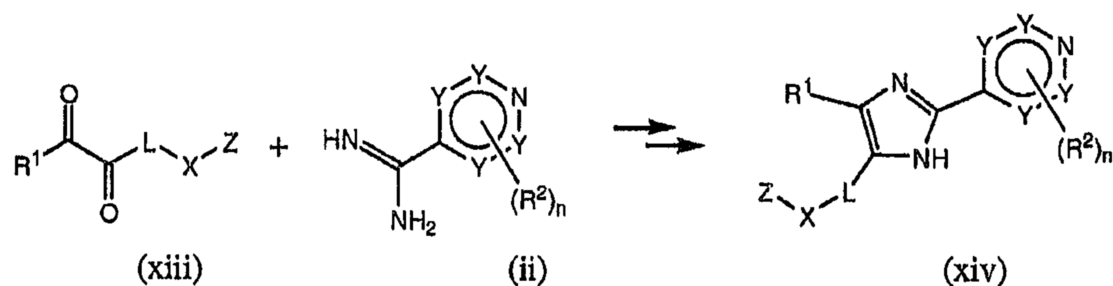
Scheme 4
