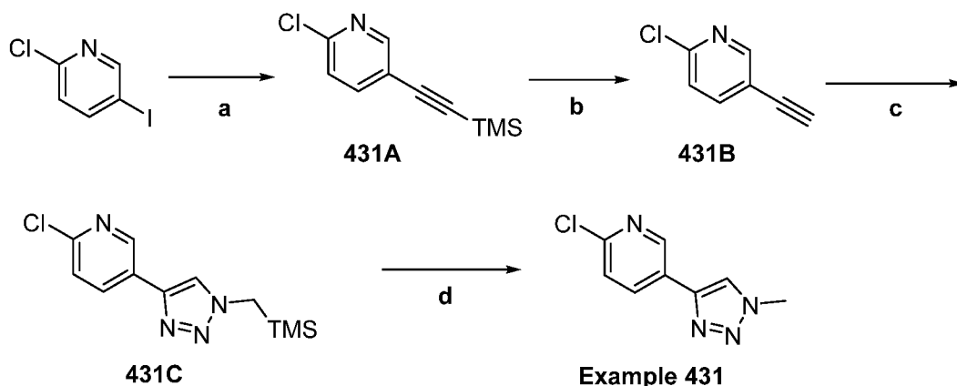
Scheme 66
