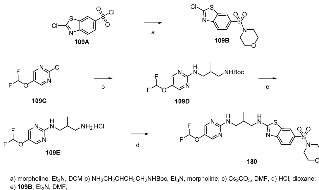
Scheme 11
