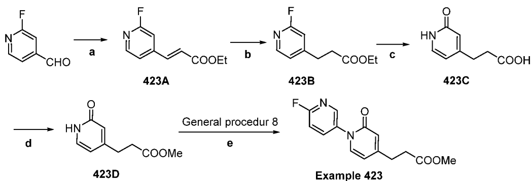
Scheme 64
