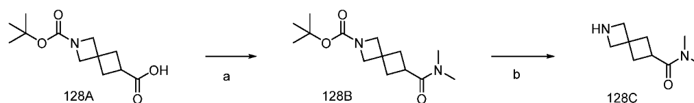
Scheme 33
