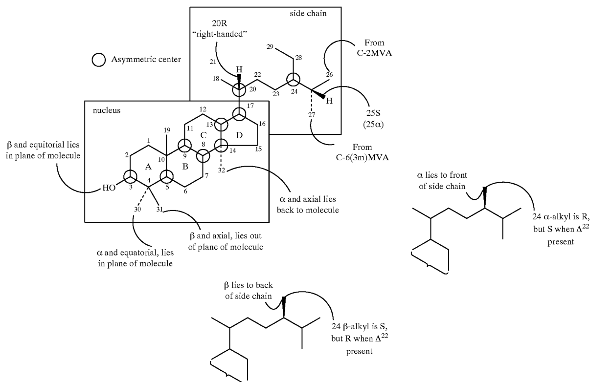
Scheme 1 (adapted from Nes and Venkatramesh, 1997)
