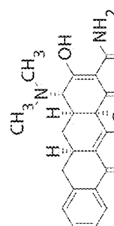
7-Aza-10-Deoxysancycline (4) (14 steps, 6.1%)
