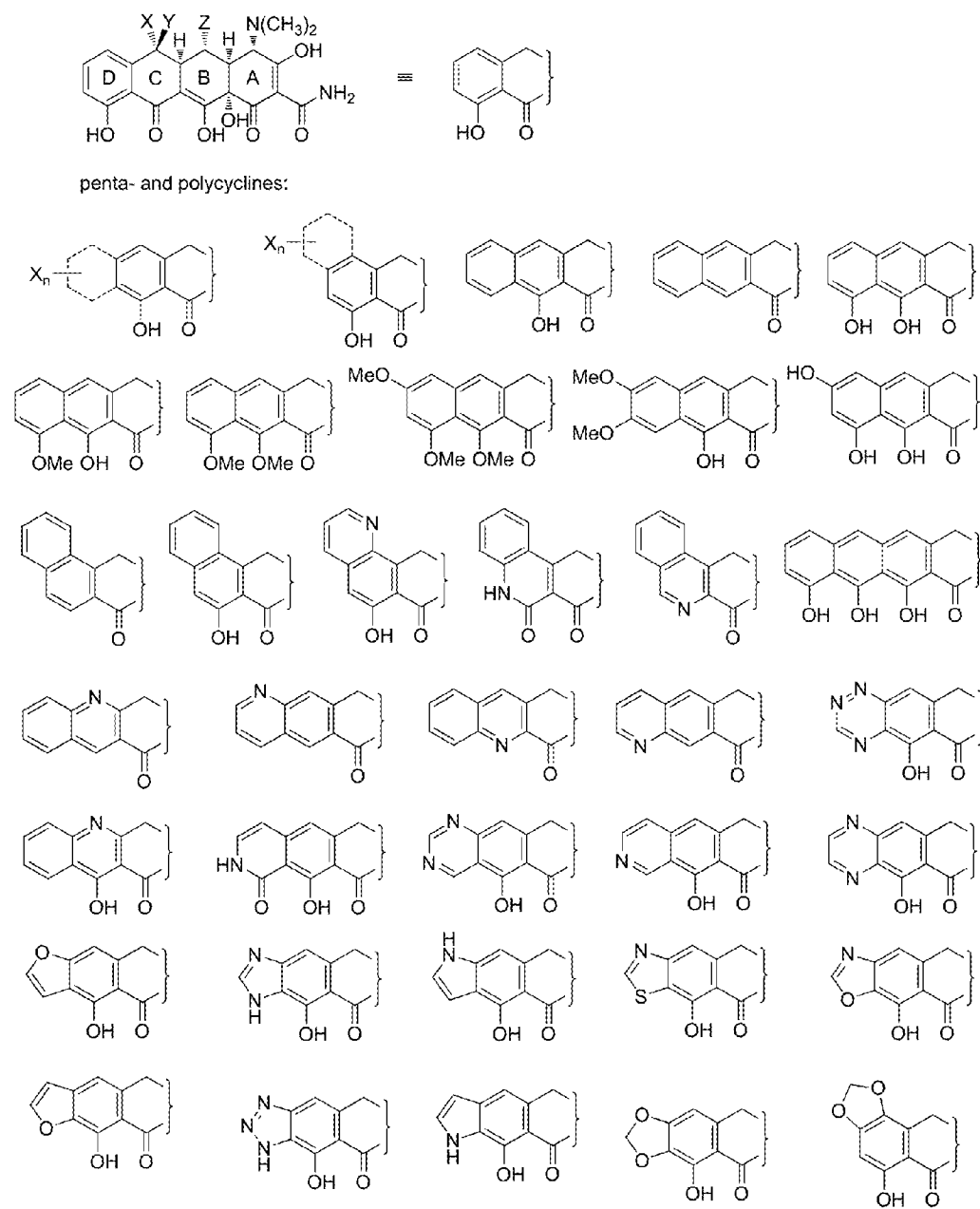
Figure 14B Representative Structures
