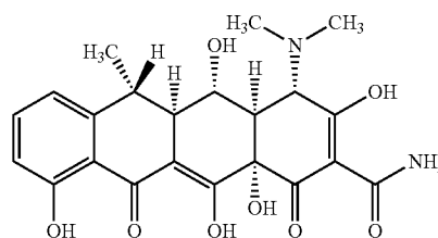
(S)-doxycycline
