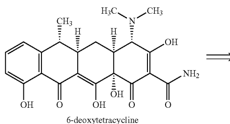
6-deoxytetracycline
