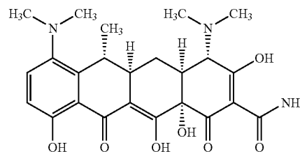
(S)-minocycline
