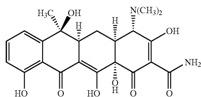
(-)-tetracycline
