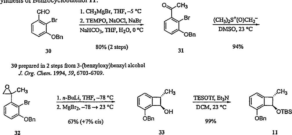
Figure 5 Synthesis of Benzocyclobutenol 11:
