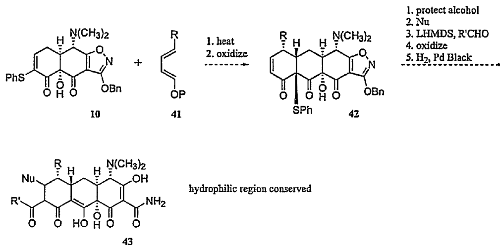
Figure 7 Summary of Targeted "Tricyclines"
