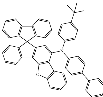
&lt;Chemical Formula 3&gt;
