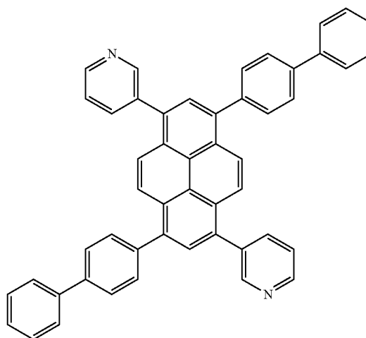
[Chemical Formula E-3]
