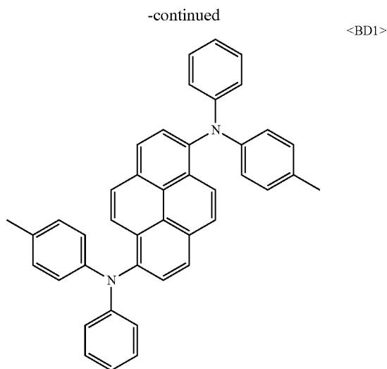
[Chemical Formula E-1]
