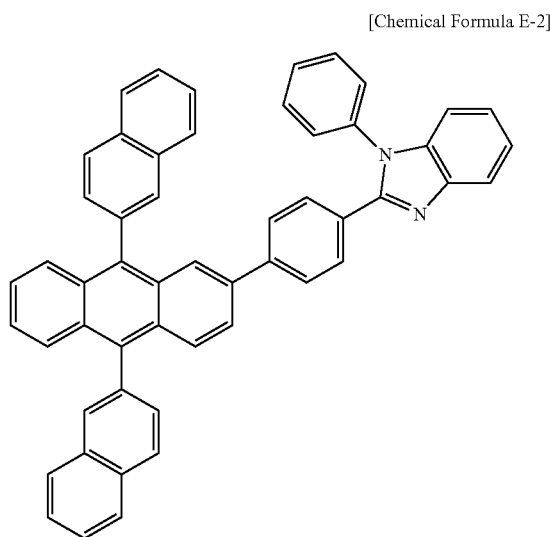
[Chemical Formula E-2]
