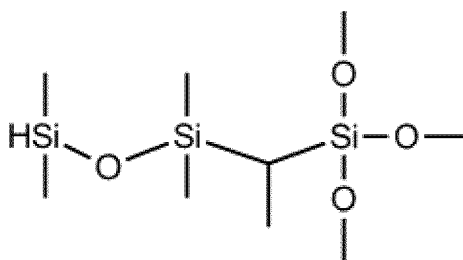
alpha-adduct
