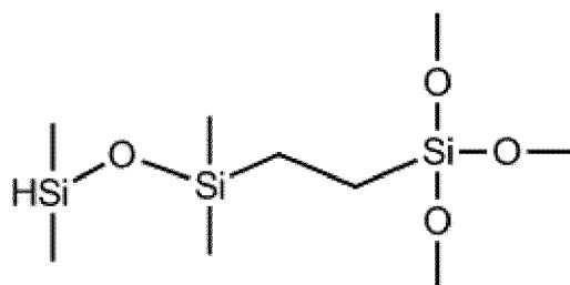
beta-adduct
