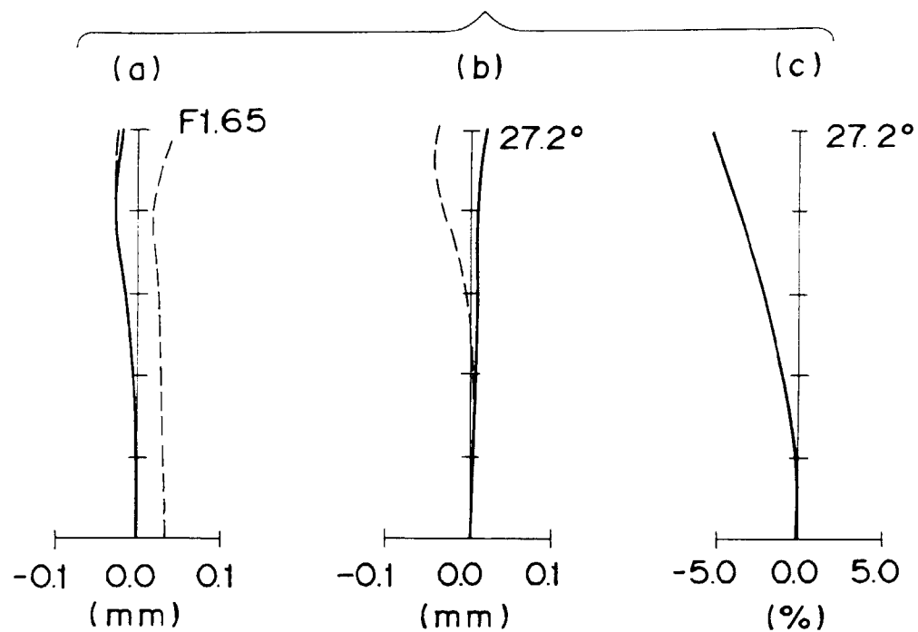
Fig. 9 ( f = 6.179 )
