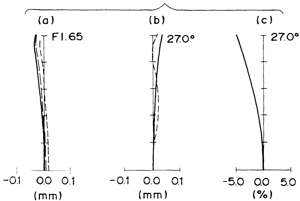
Fig. 13 ( f = 6.178 )
