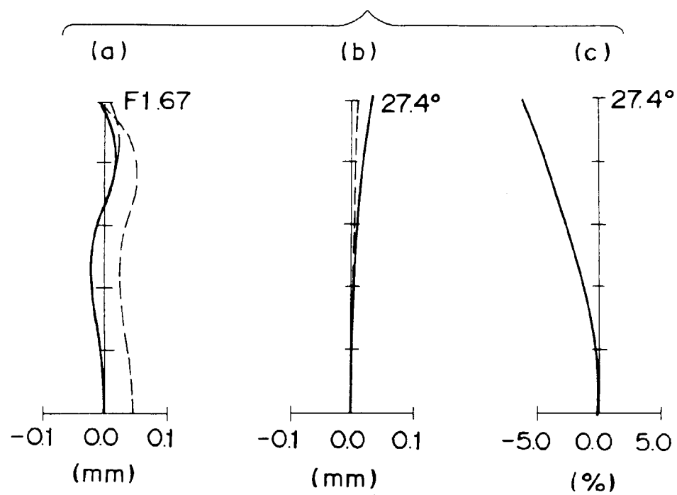
Fig. 6 ( f = 6.161 )
