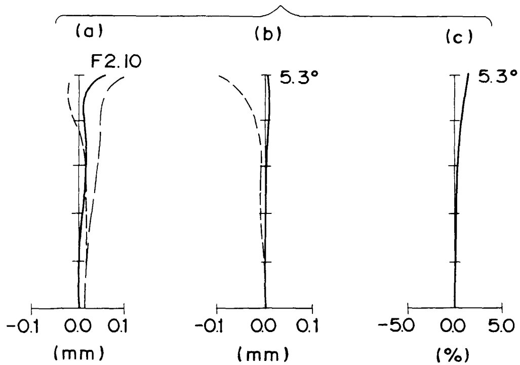
Fig. 14 ( f = 31.727 )
