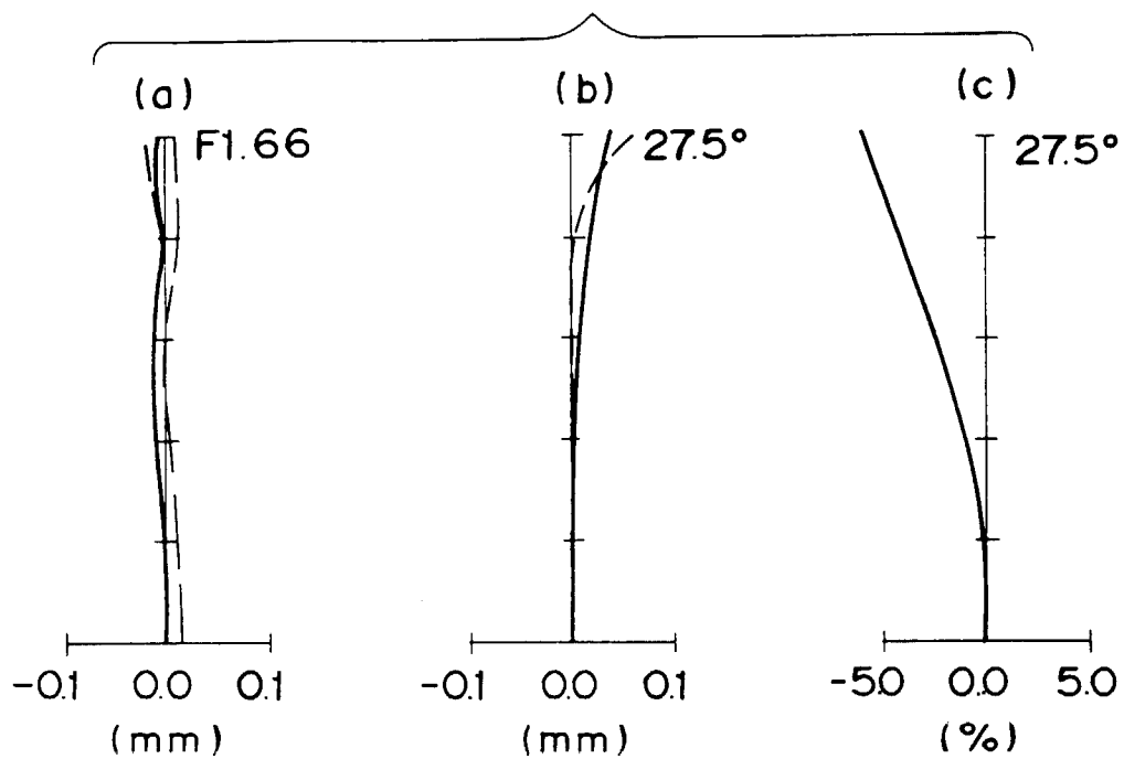
Fig. 3 ( f = 6.140 )
