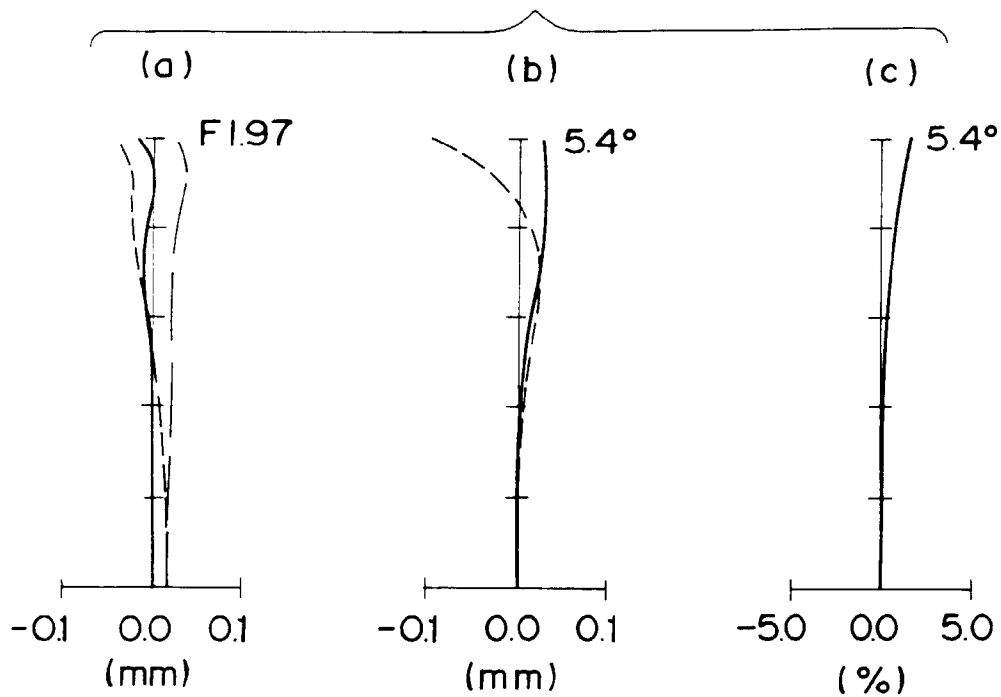
Fig. 10 ( f = 31.422 )
