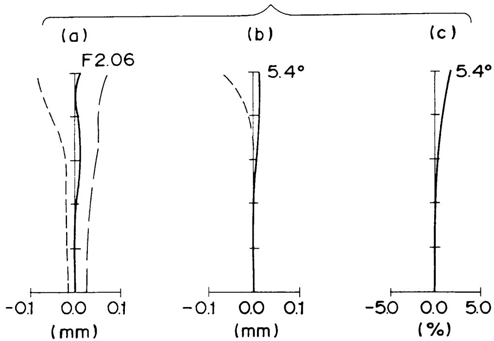
Fig. 4 ( f = 31.286 )
