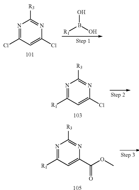
Reaction Scheme 1
