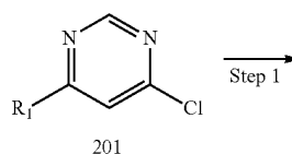
Reaction Scheme 2
