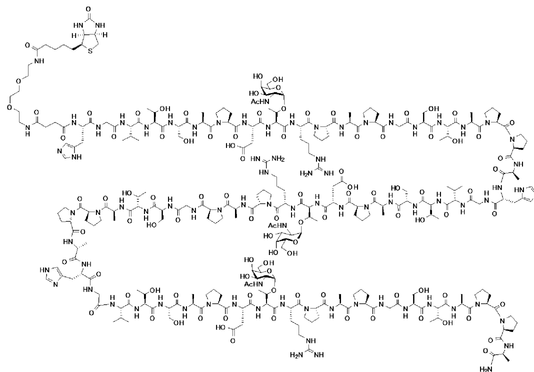
Compound 20
