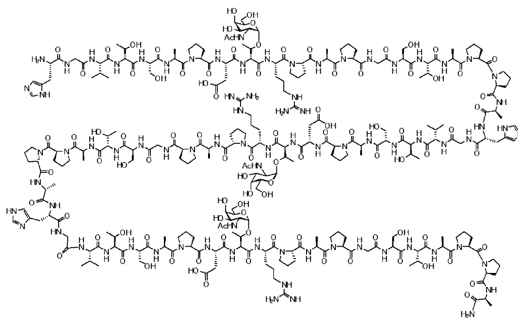
Compound 15
