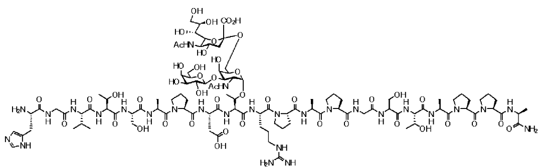
Compound 11
