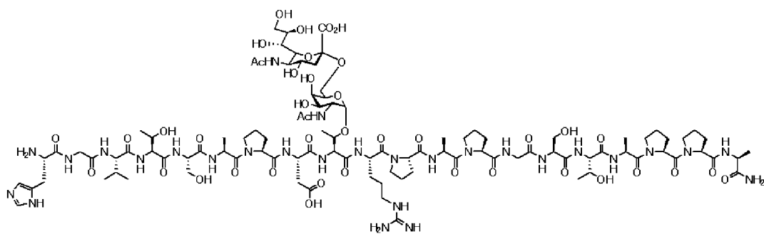
Compound 5
