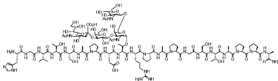
Compound 7
