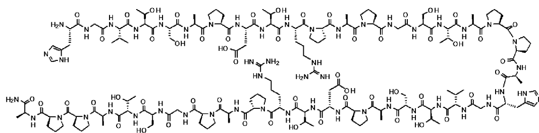
Compound 14
