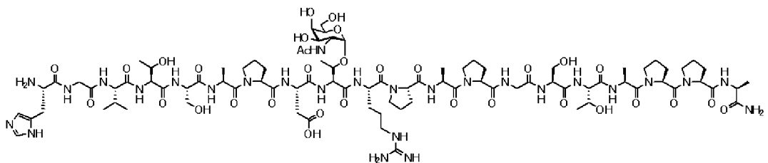
Compound 4
