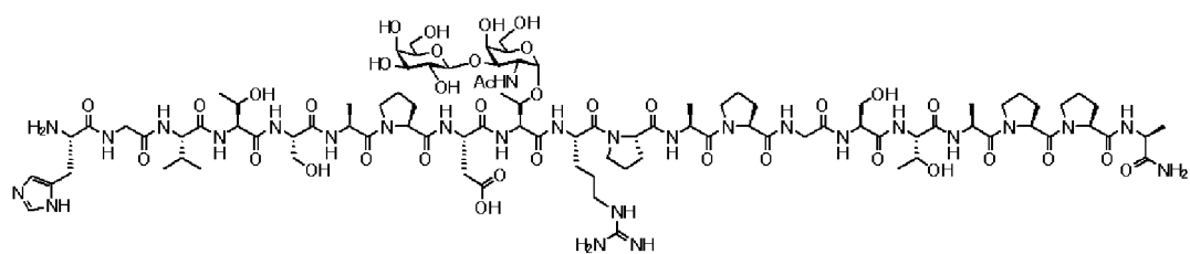
Compound 2
