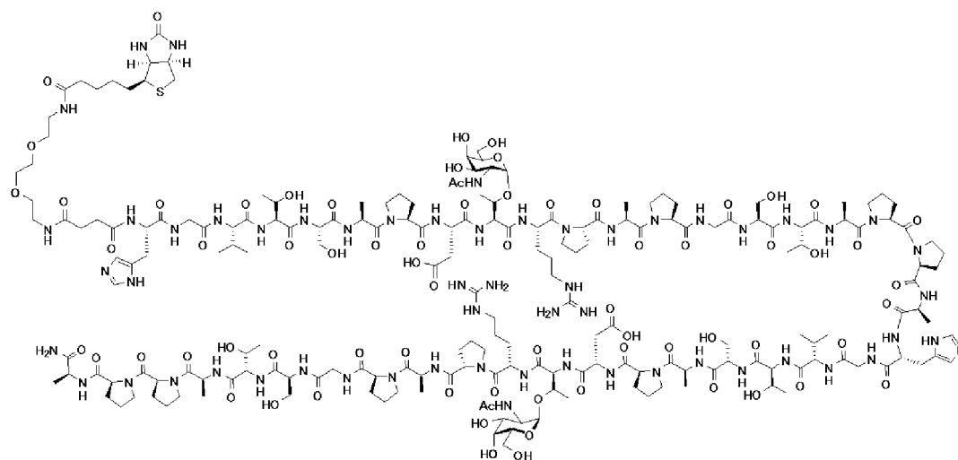
Compound 19
