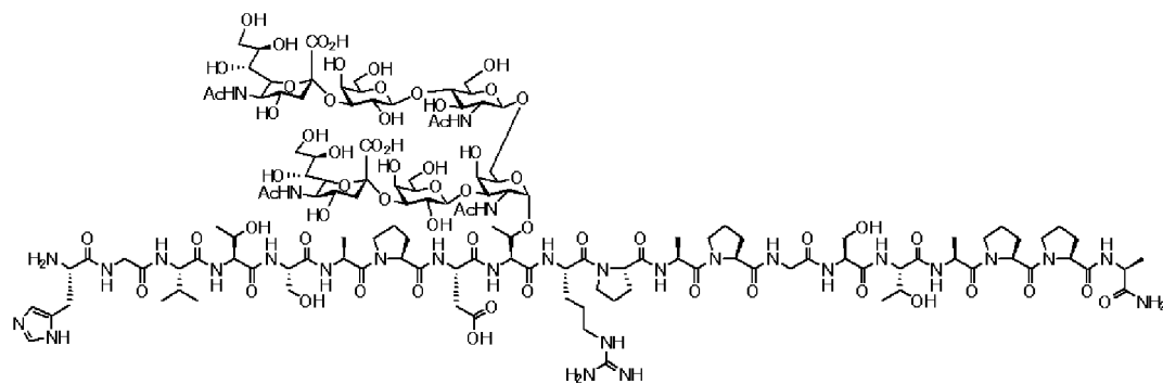
Compound 9
