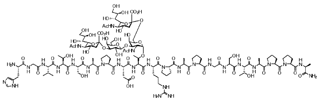
Compound 12
