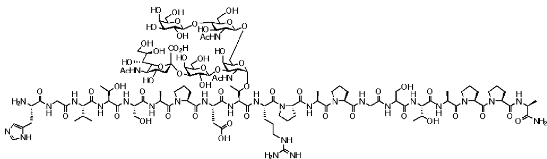
Compound 8
