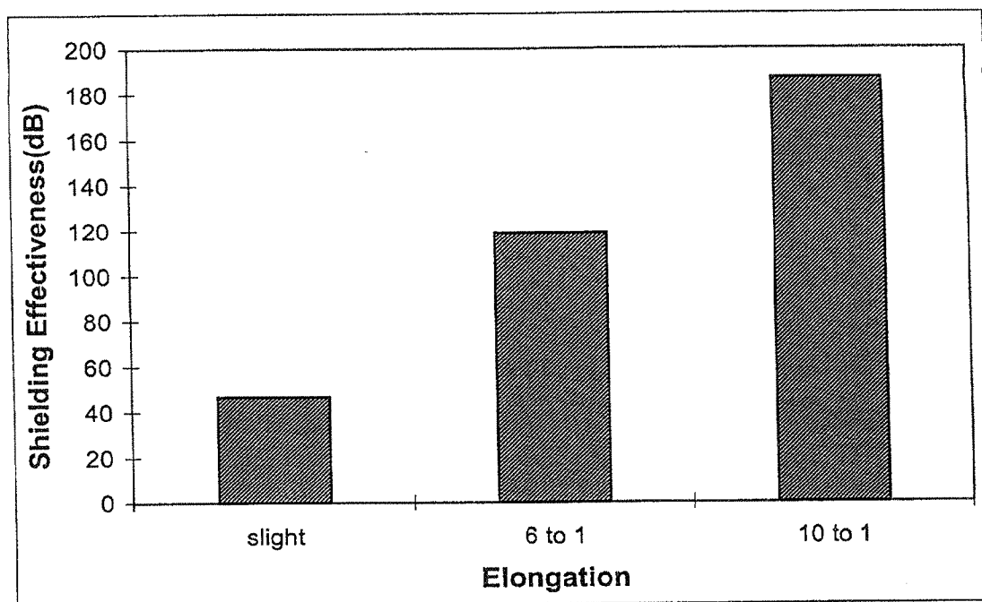
FIG. 1. EM Shielding Effectiveness as a function of shear load of 1.5% nanotube containing PET.
