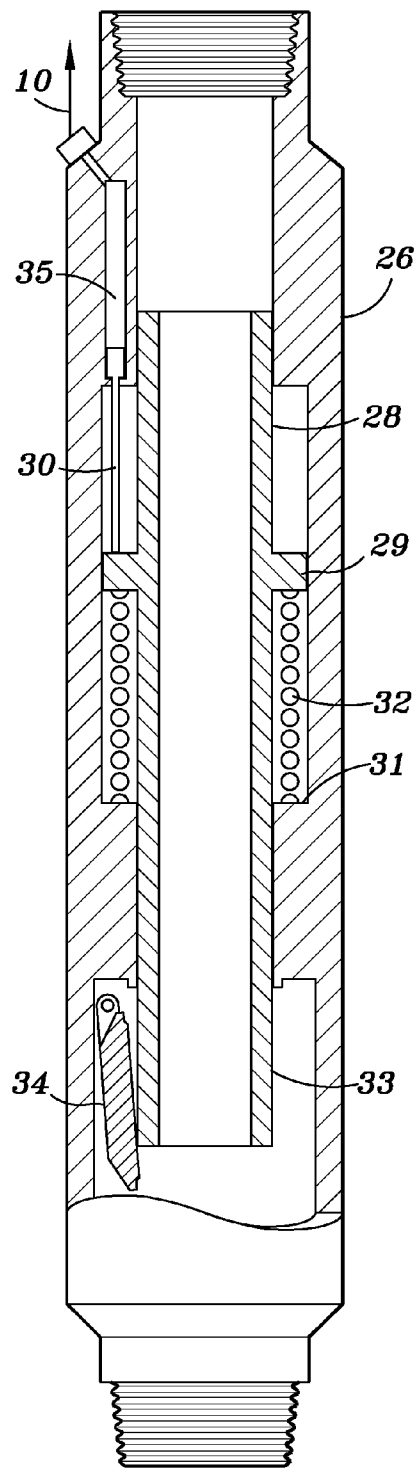
PRIOR ART FIG. 2B
